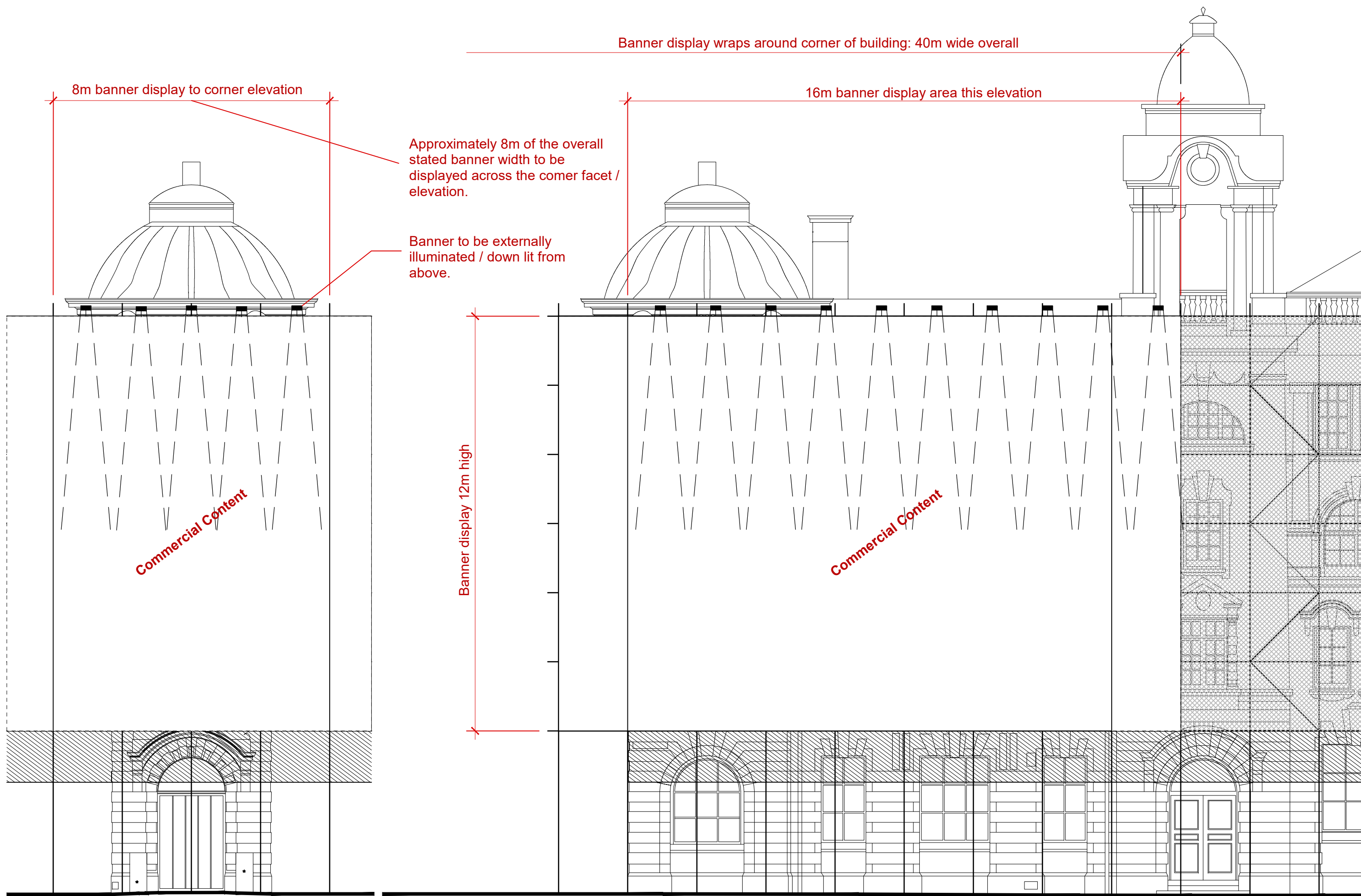
Corner Elevation
