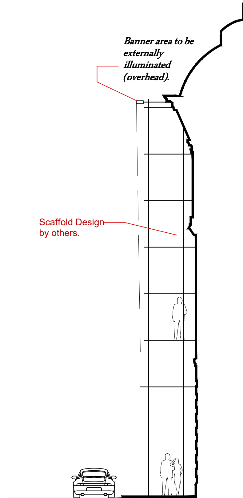
Typical Section
