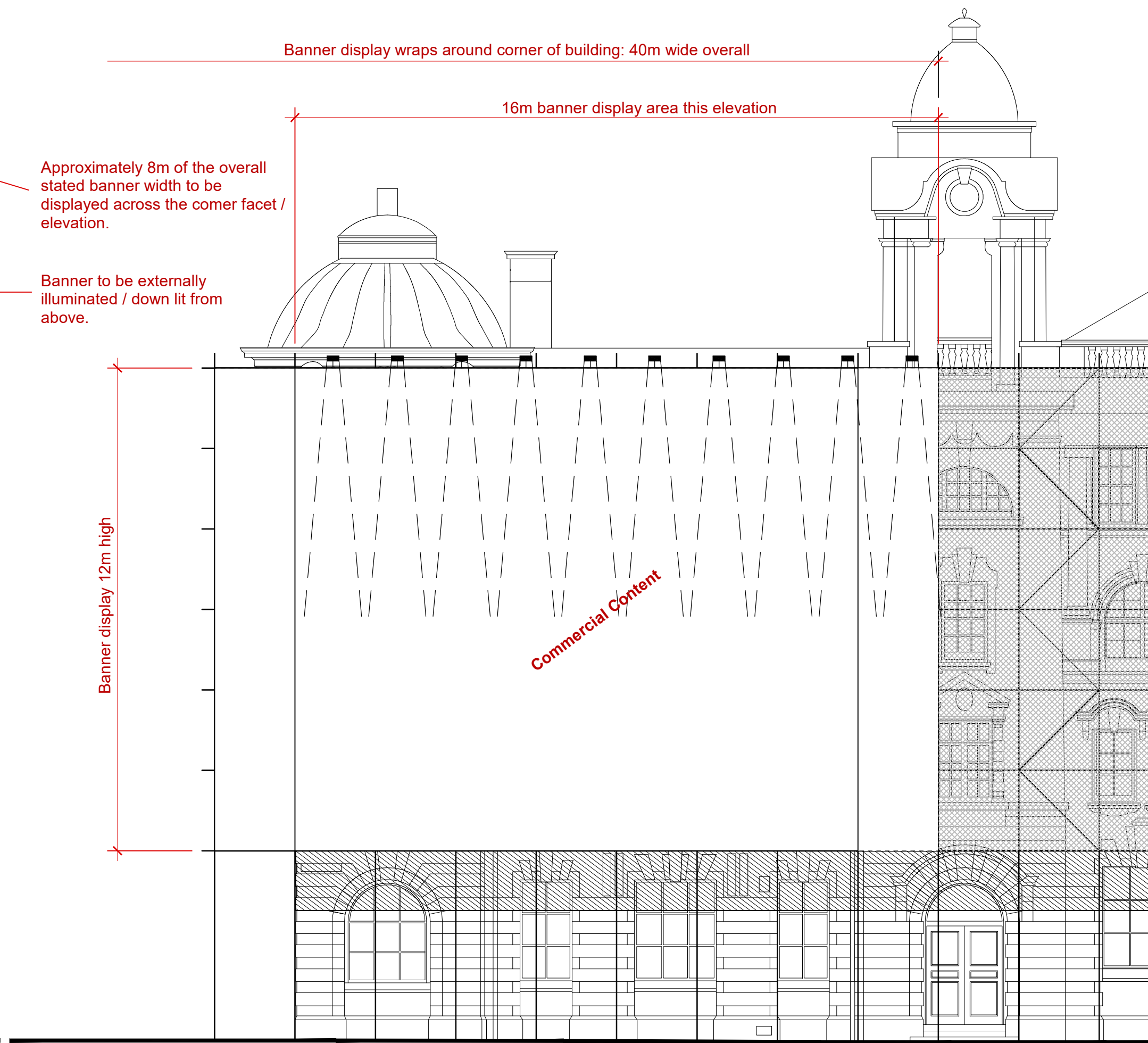
London Road Elevation
