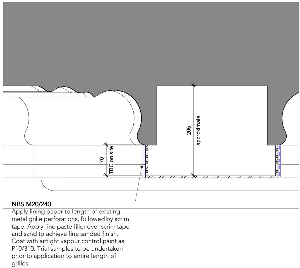
3 Callout Detail_Downstand beams, Metal Grille Treatment 1 : 5
