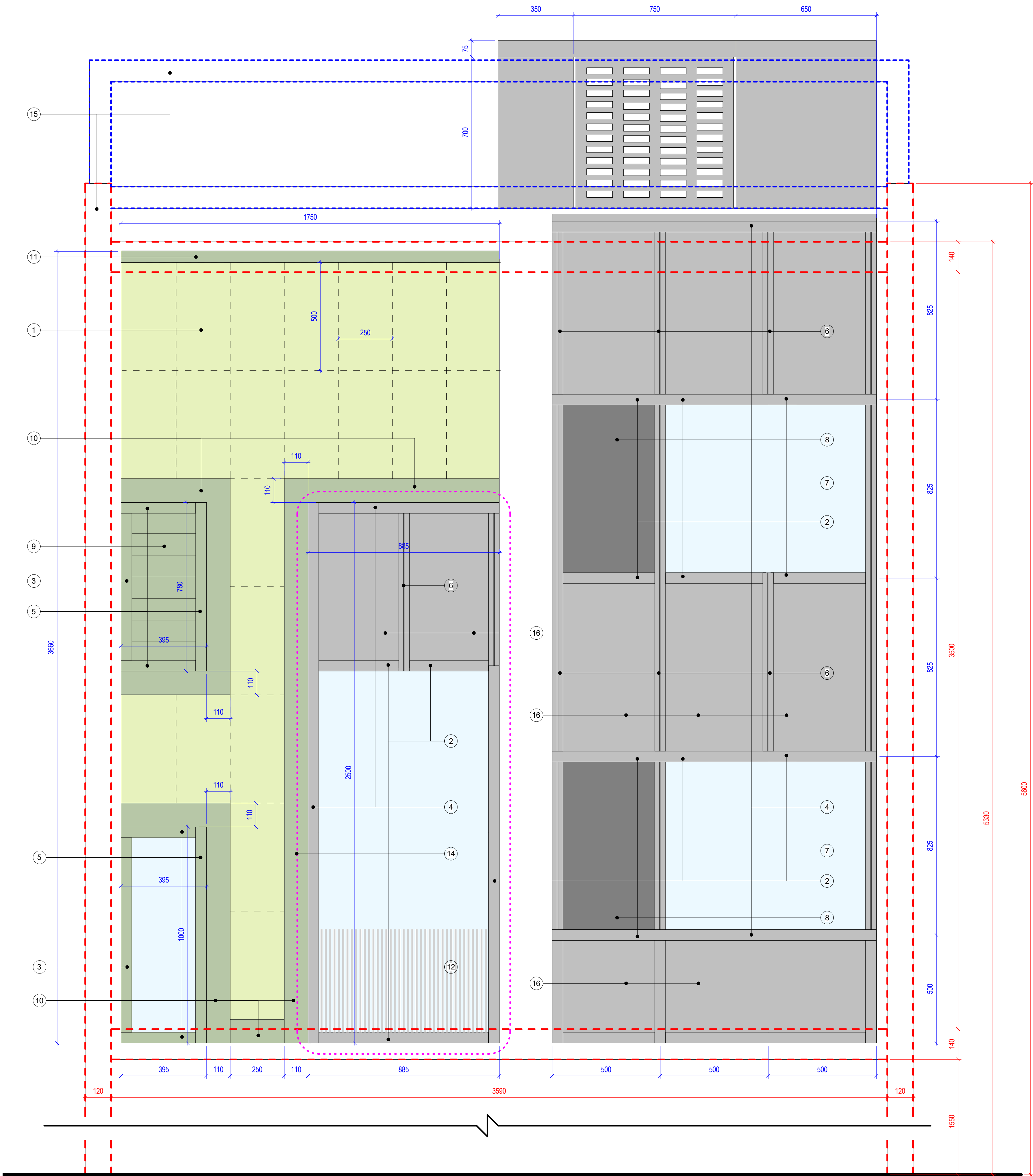
1 Mock Up Elevation 1:10
