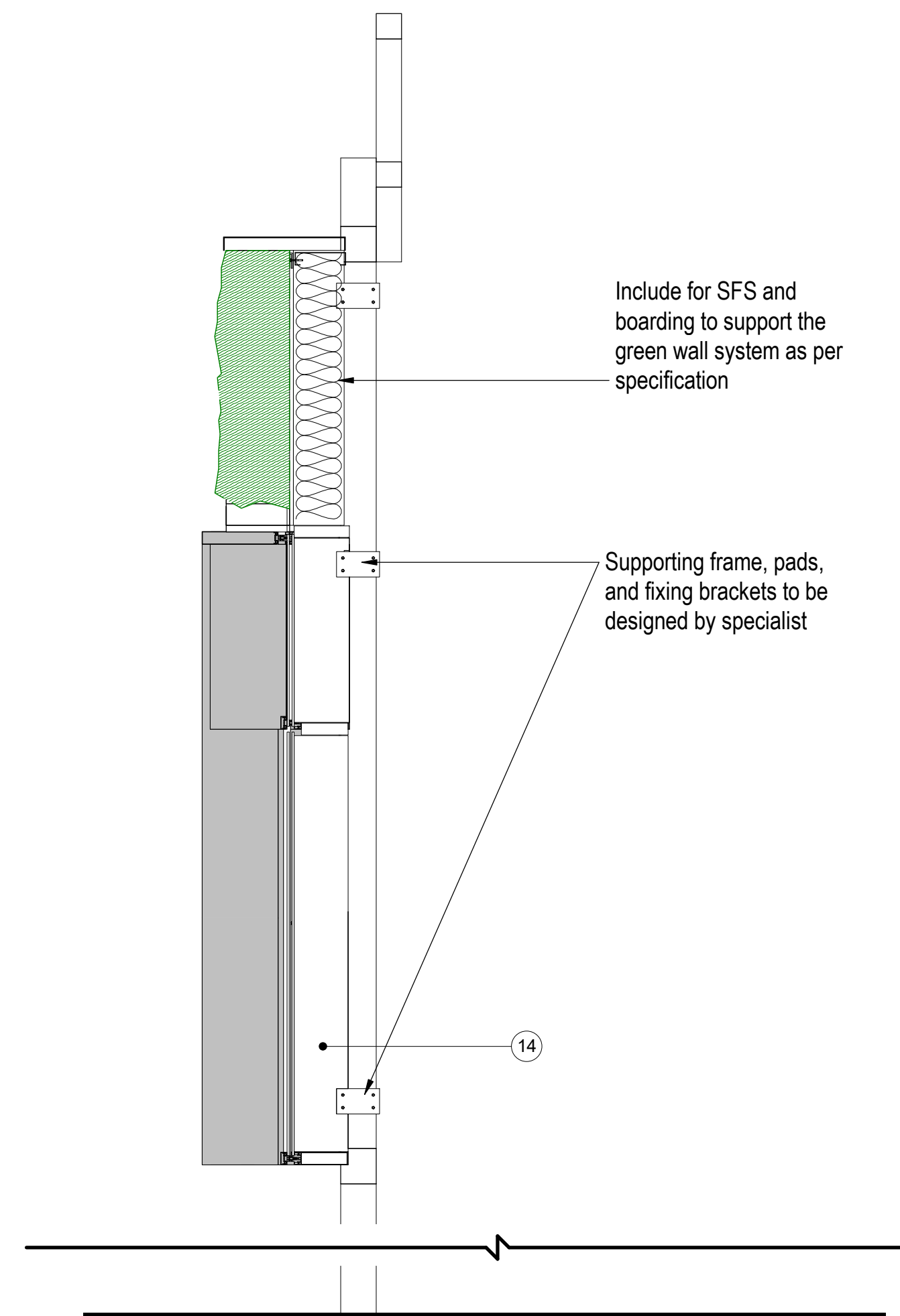
2 Mock Up Elevation including planting 1:25
