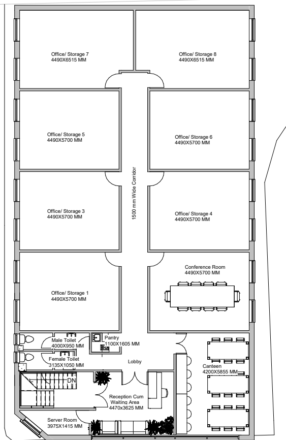
2 First Floor Level 1 : 100
