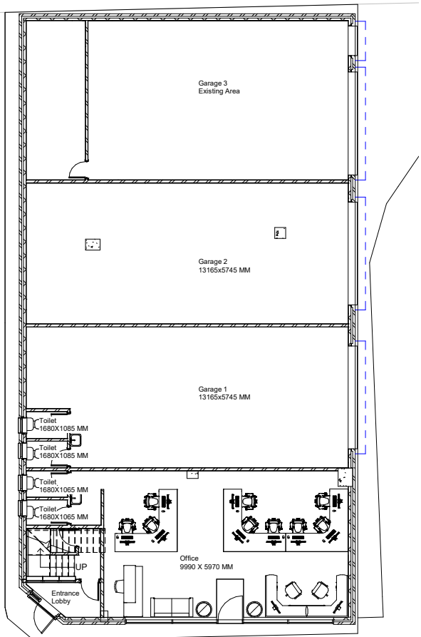
1 Ground Floor Level 1 : 100
