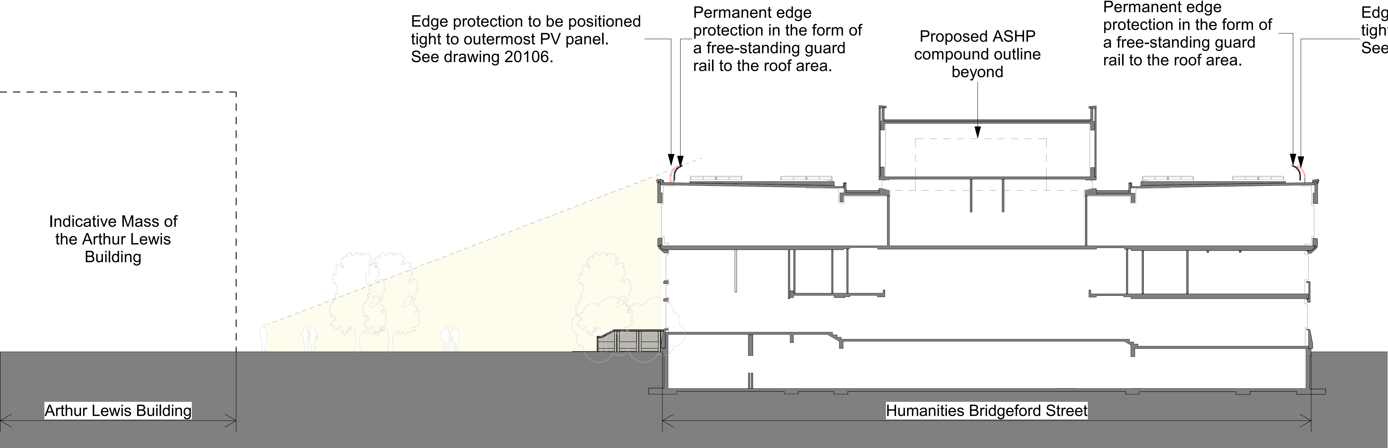
Proposed Site Section AA
