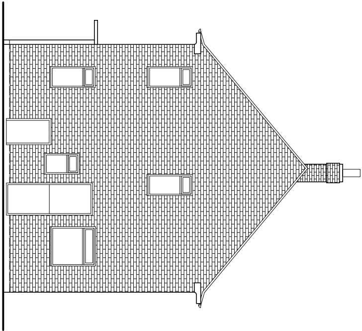
EXISTING SOUTH WEST ELEVATION
