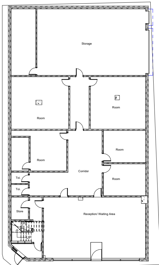
1 Ground Level 1 : 100
