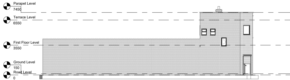
5 West Side Elevation 1 : 100
