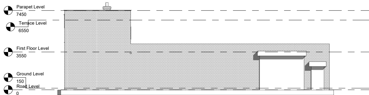
6 East Side Elevation 1 : 100
