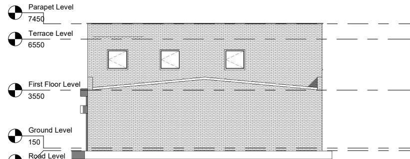
7 Rear Elevation 1 : 100
