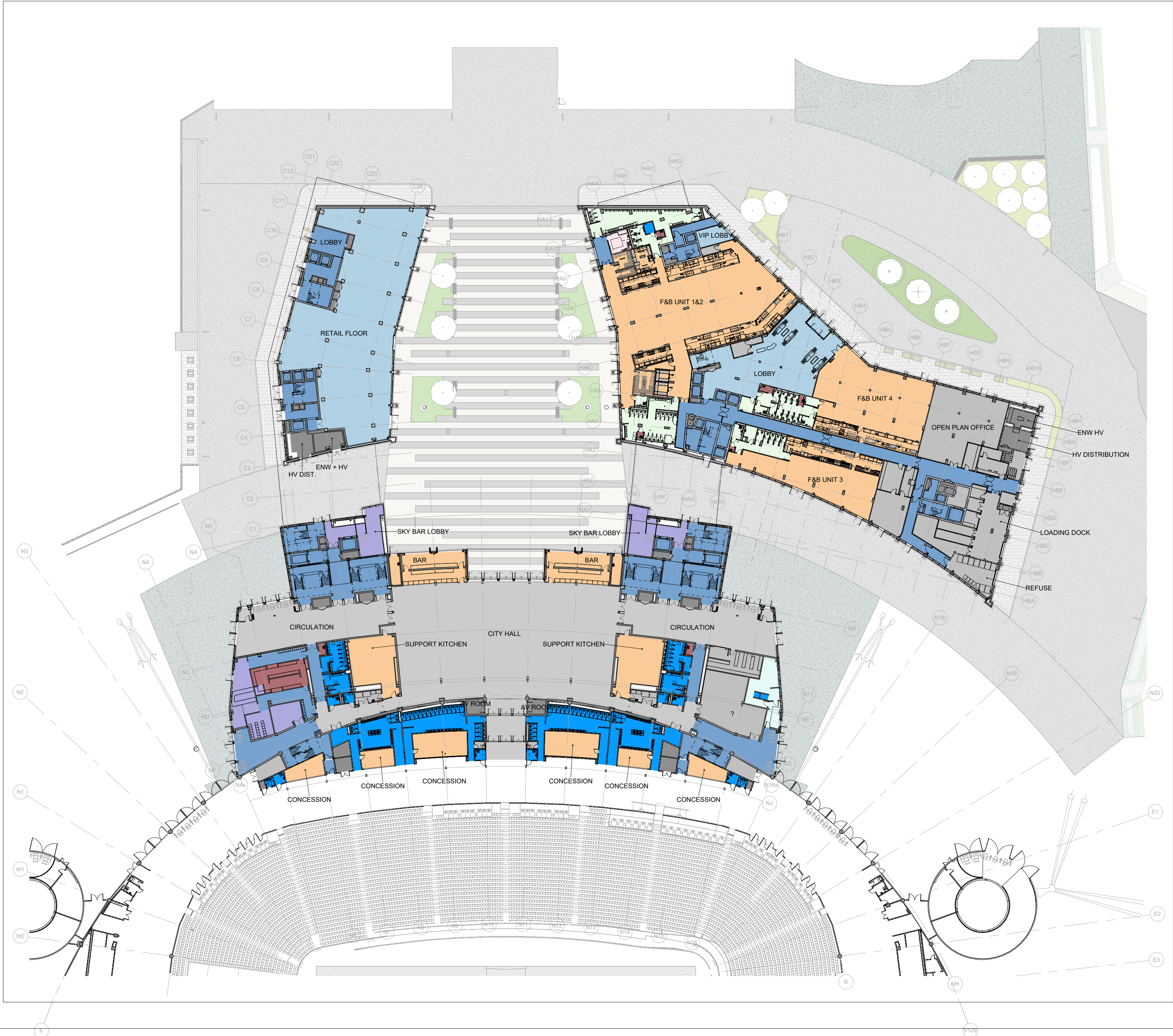
KEY PLAN
