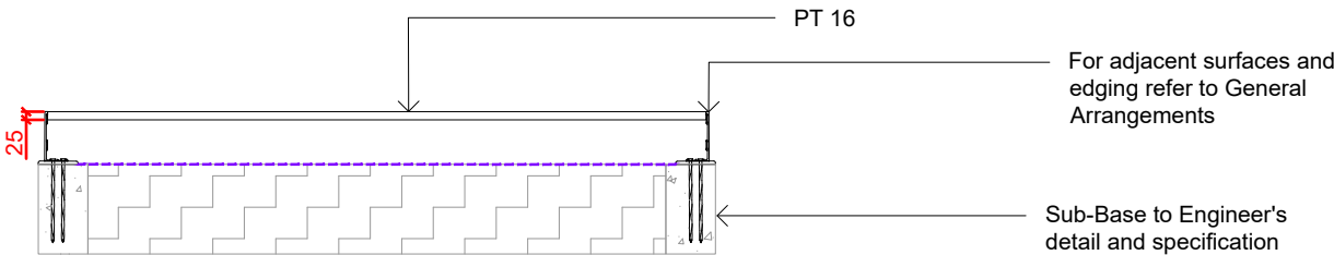
PT16 TYPICAL DETAIL 001 SECTION @ 1:25
