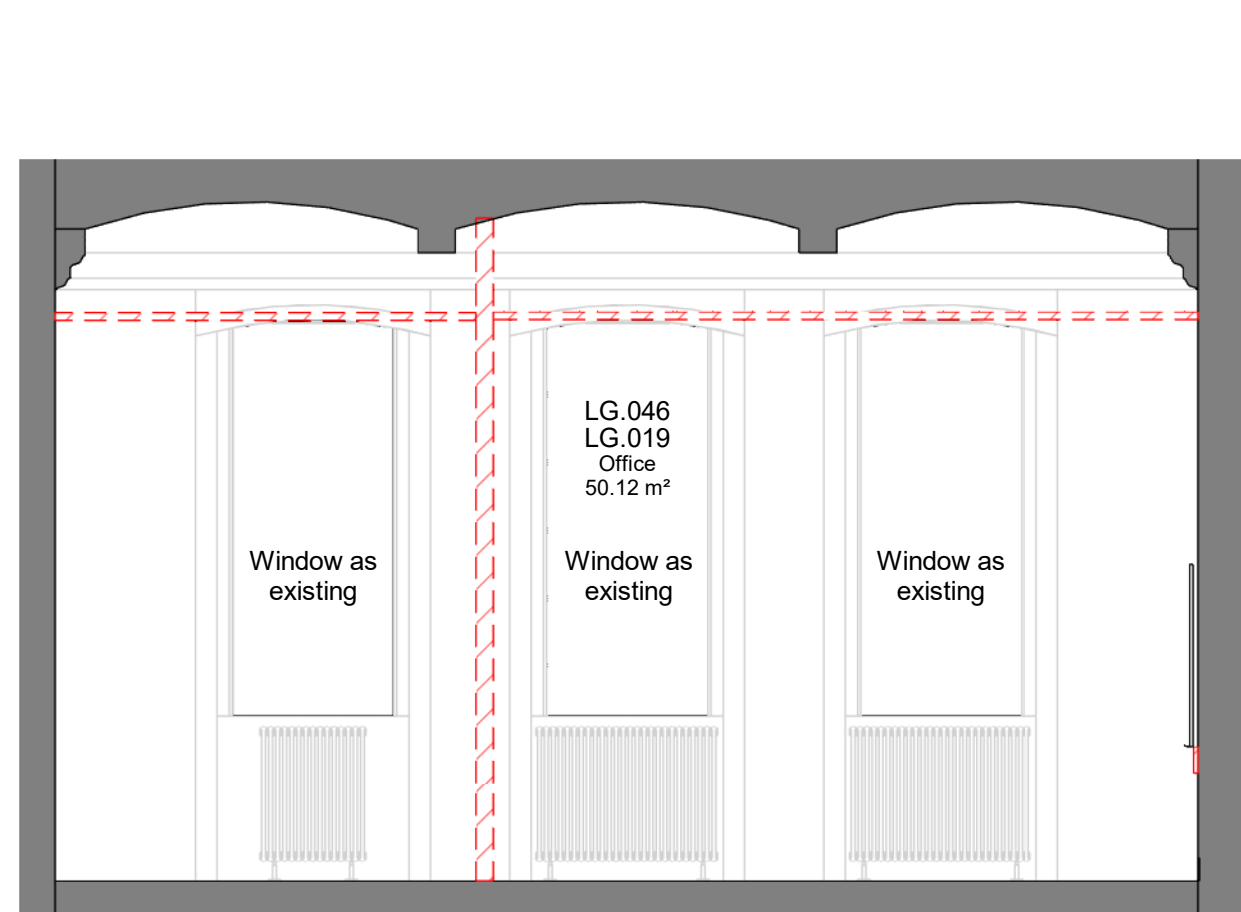
LG.019 Elevation A
