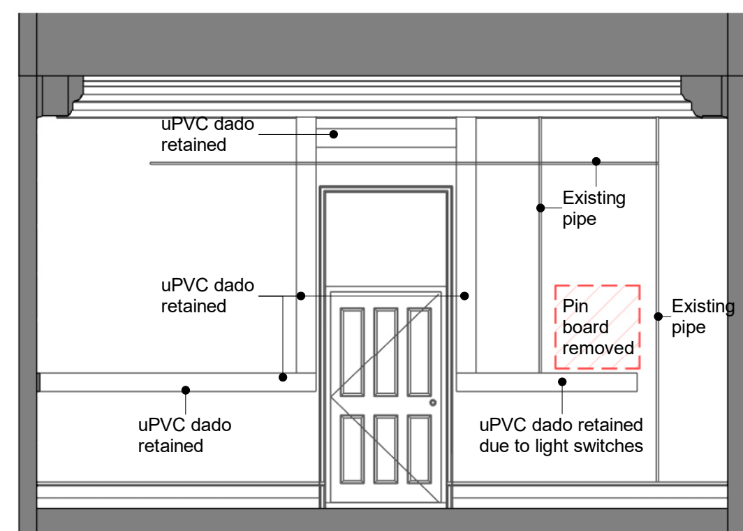
LG.005 Elevation G
