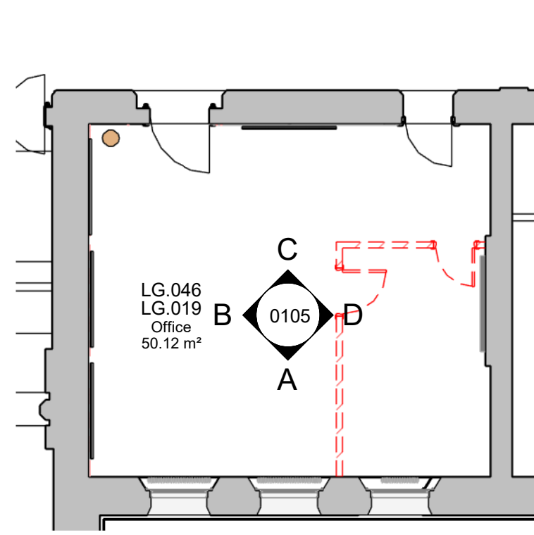
LG.019 Layout
