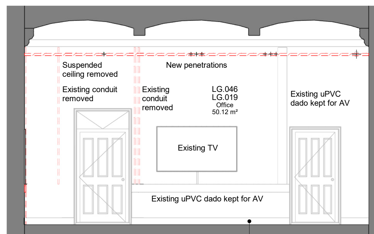
LG.019 Elevation C
