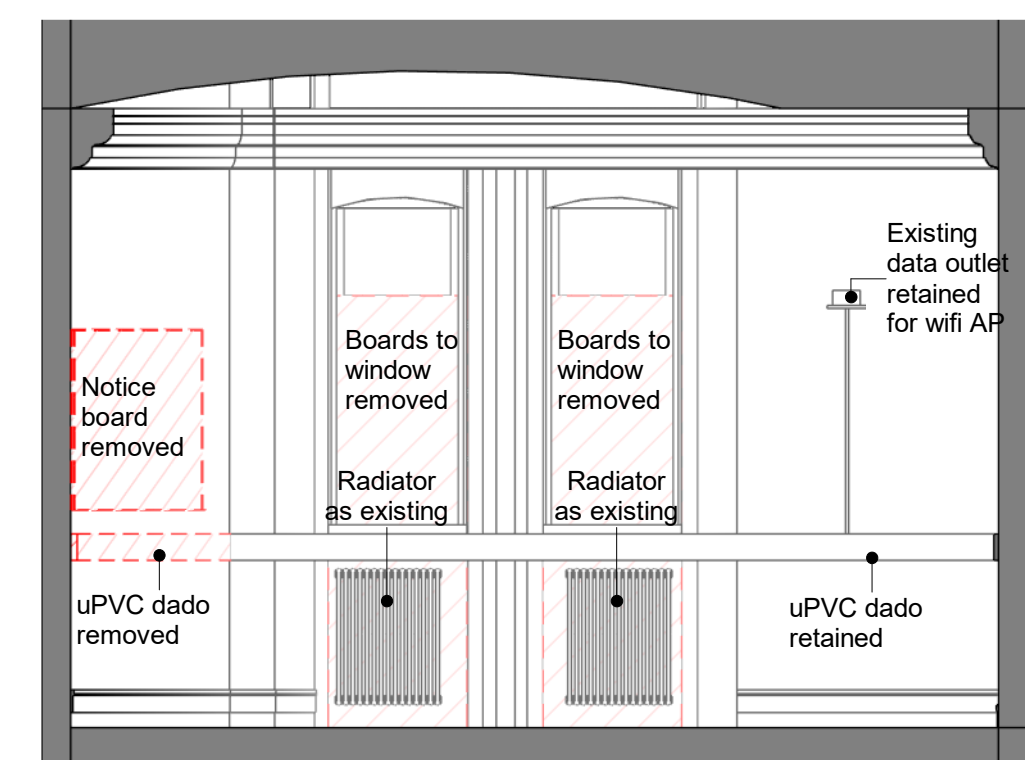
LG.005 Elevation H
