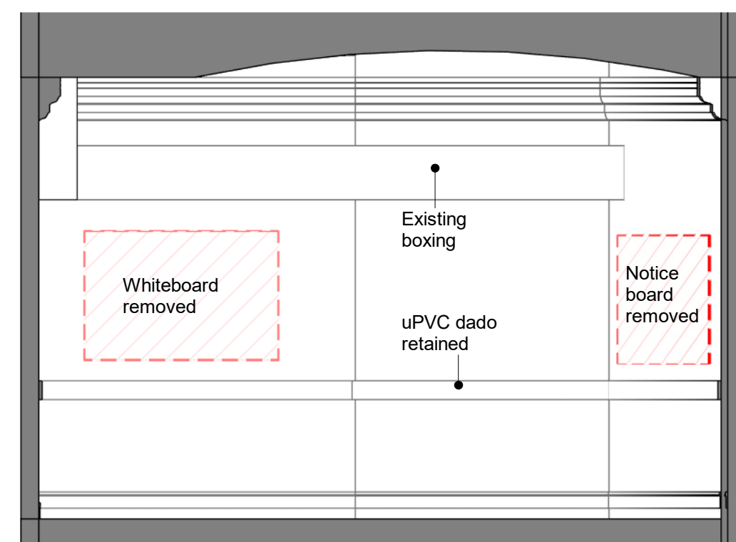
LG.005 Elevation F
