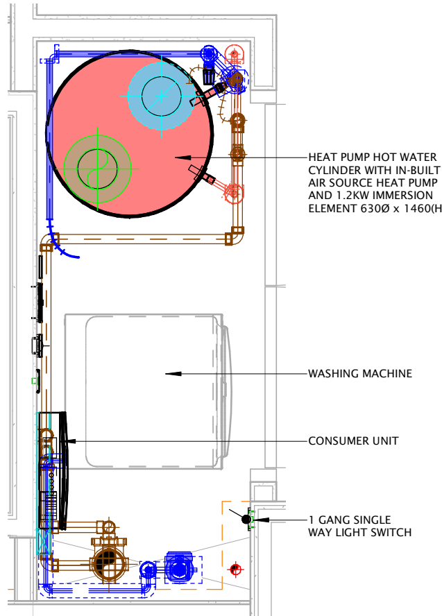
Type 01 - Combined Services Low Level 1 : 20
