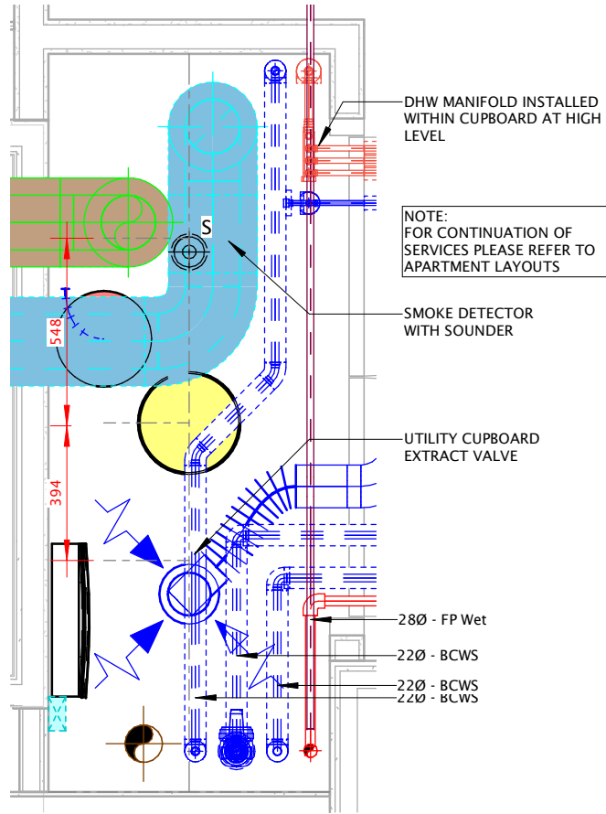
Type 01 - Combined Services High Level 1 : 20
