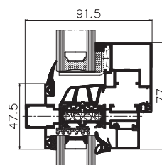
fixed and opening window – cross section
