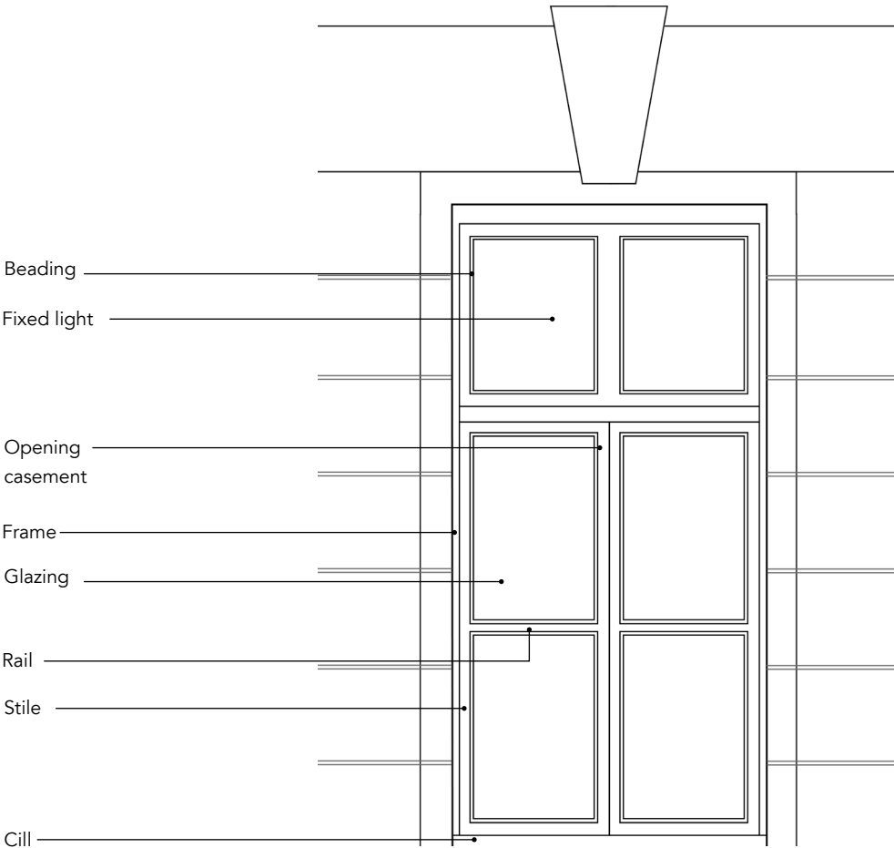
Typical French Window with Fixed Top Light to Athenaeum Building Drawing
