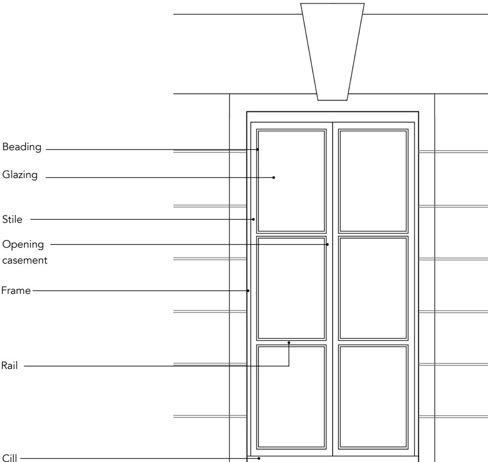
Typical French Windows to Athenaeum Basement Drawing
