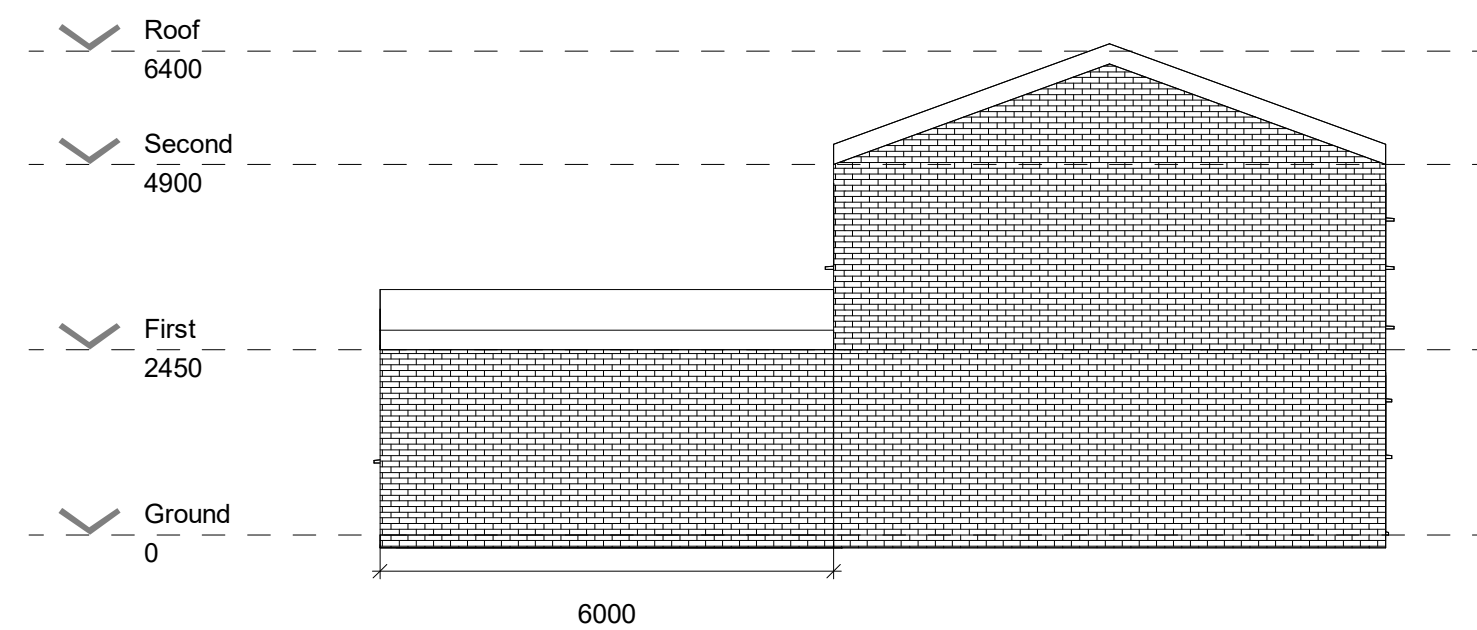
4 Proposed East Elevation
