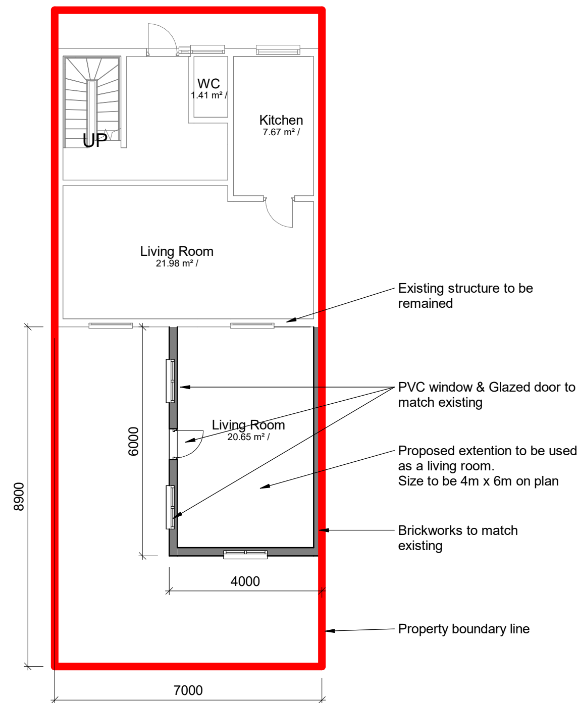
1 Proposed Ground Floor Plan
