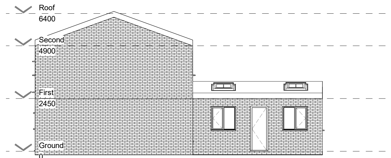
6 Proposed West Elevation
