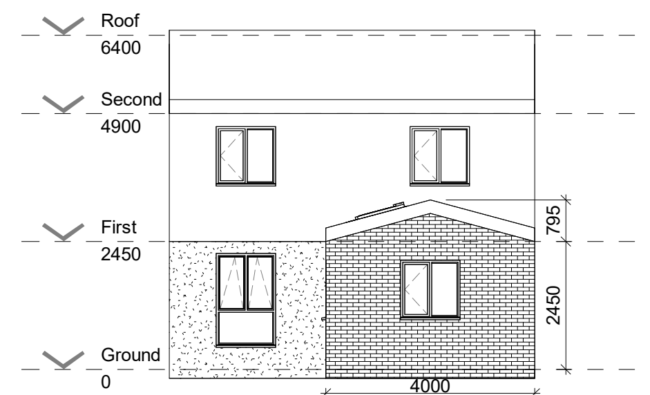
5 Proposed South Elevation
