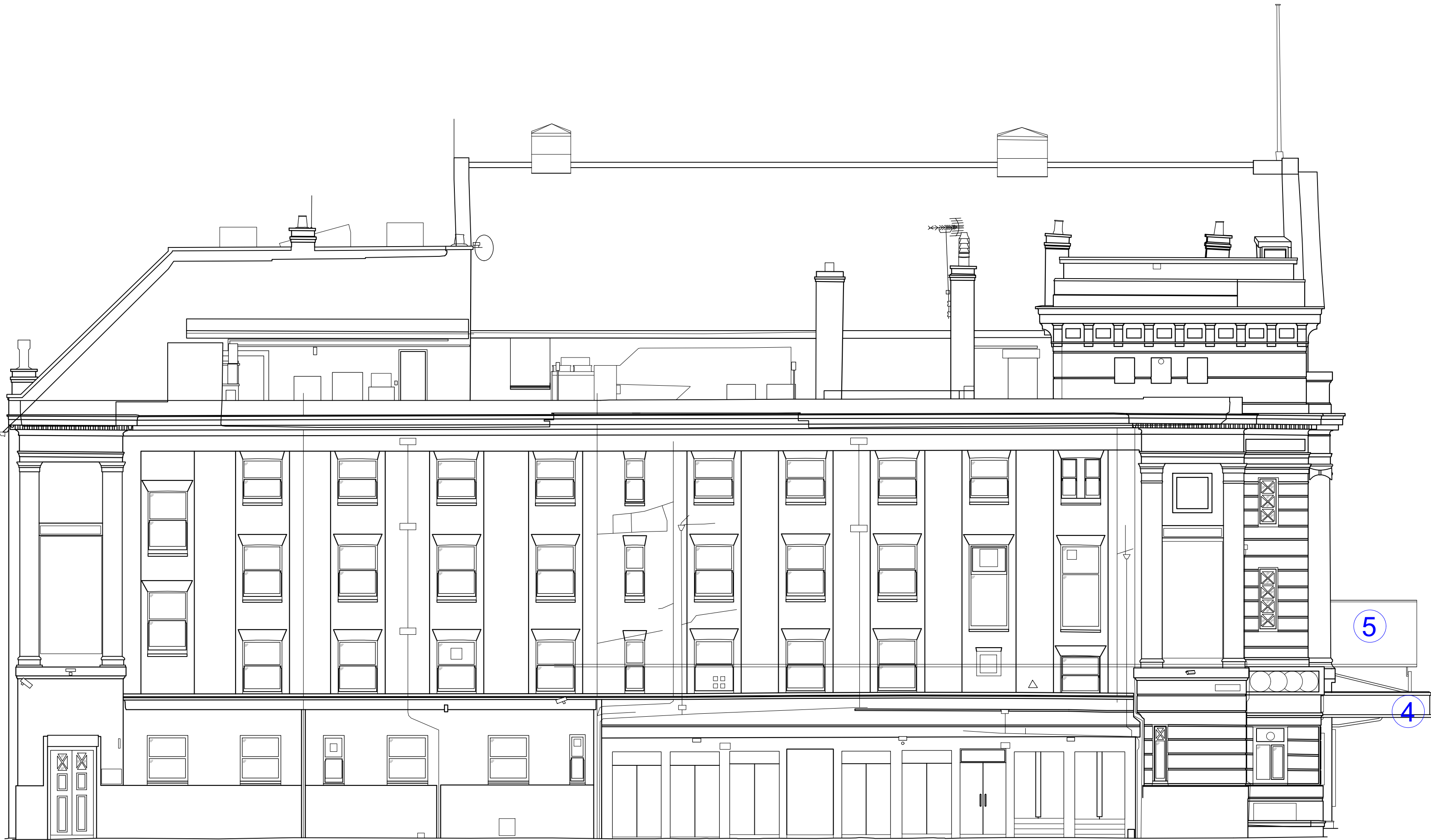
EXISTING BYROM STREET ELEVATION 1:100
