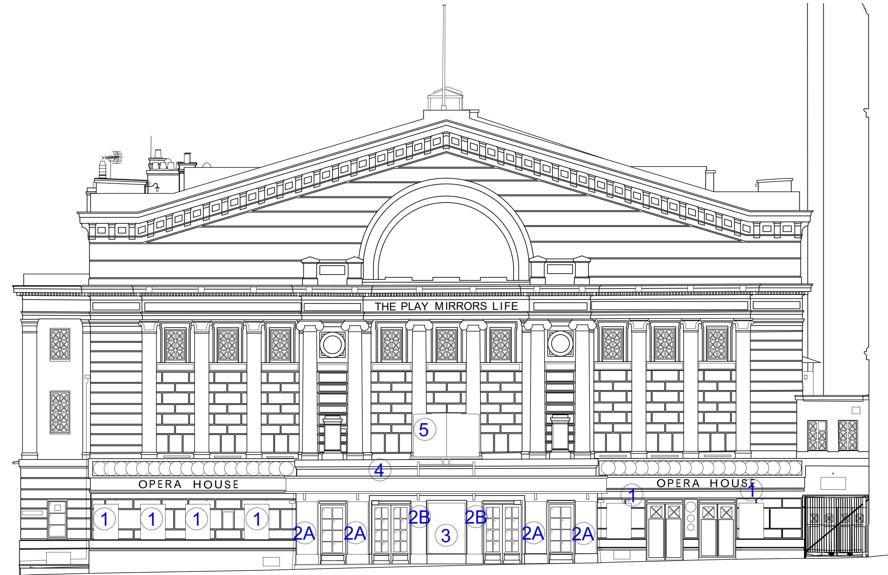
EXISTING QUAY STREET ELEVATION 1:100
