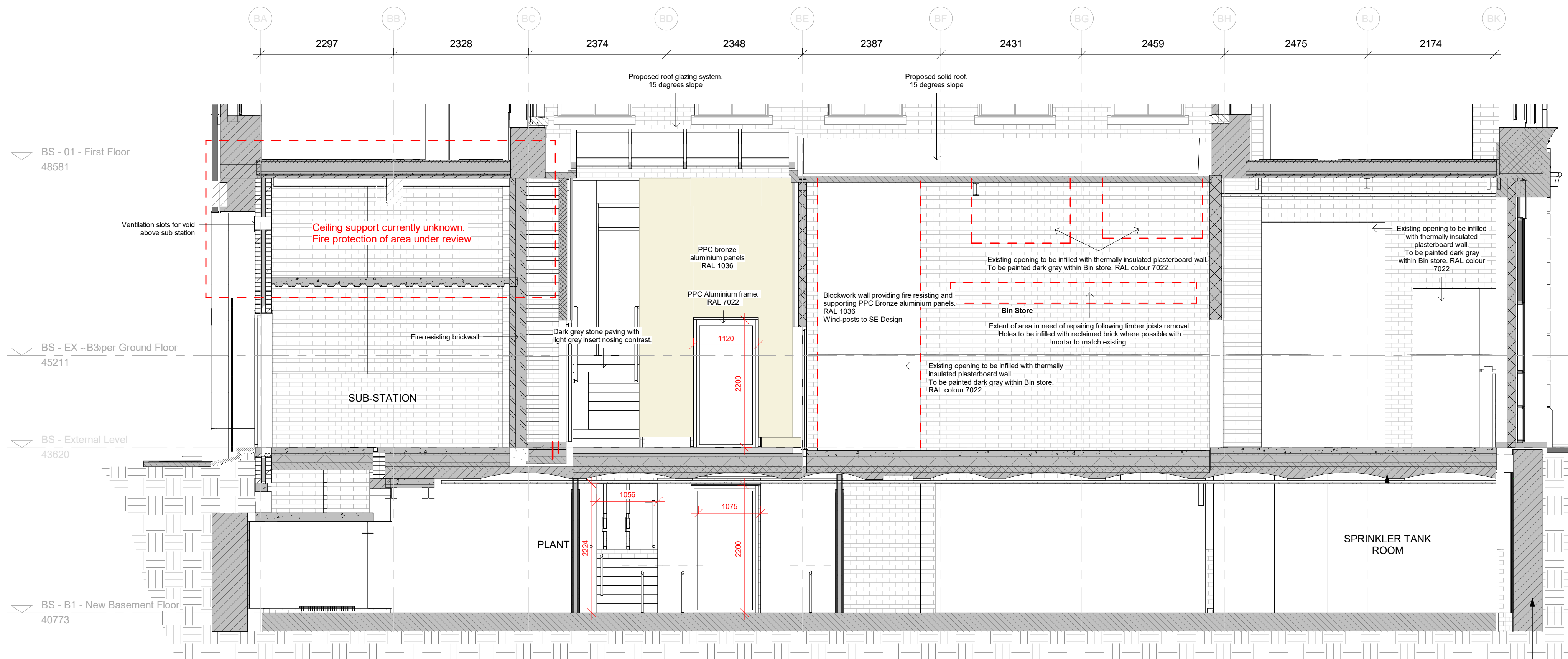
2 | Alleyway Design Intent - Long Section Copy 1
