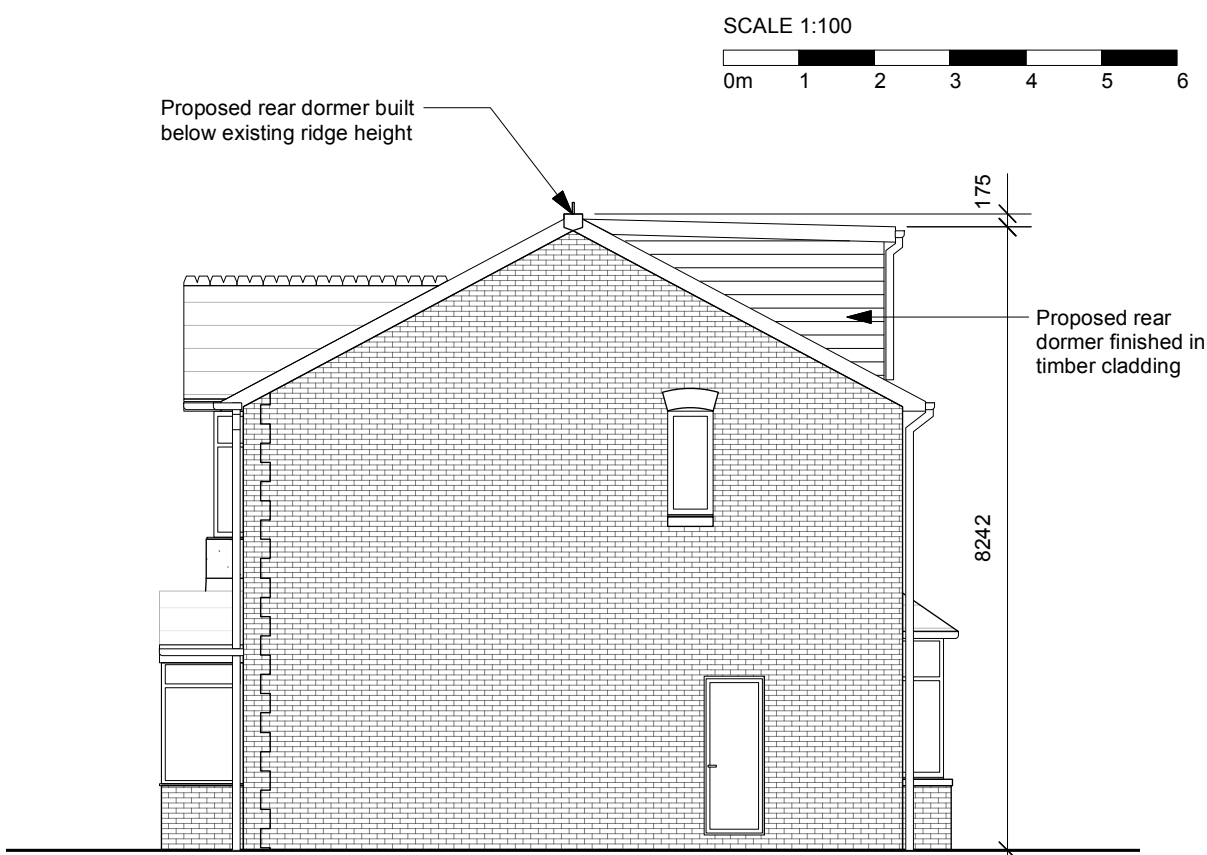
NORTH (SIDE) ELEVATION
