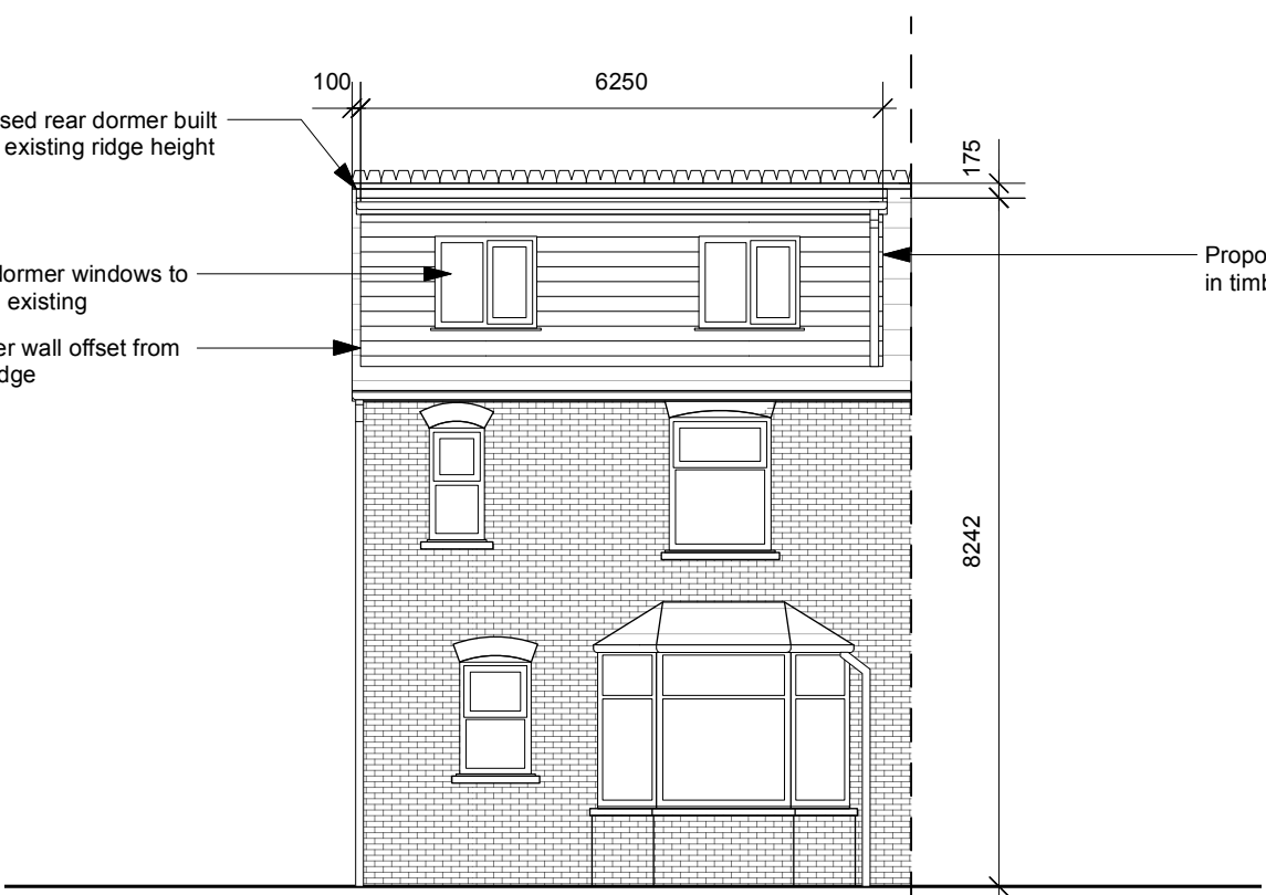
NORTH WEST (REAR) ELEVATION
