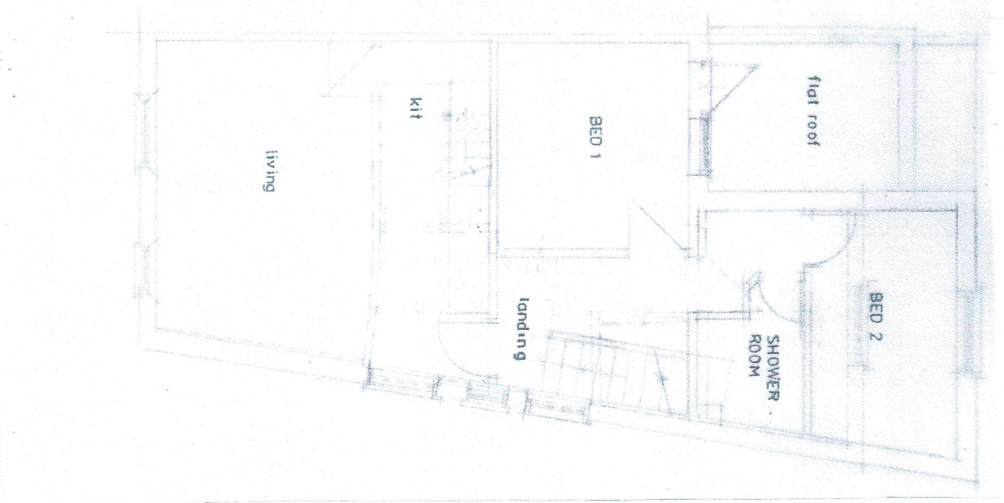
FIRST 1.100
