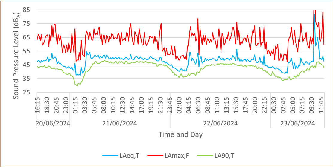
Figure 6: Long Term Survey Façade Data for the Rear Ground Floor
