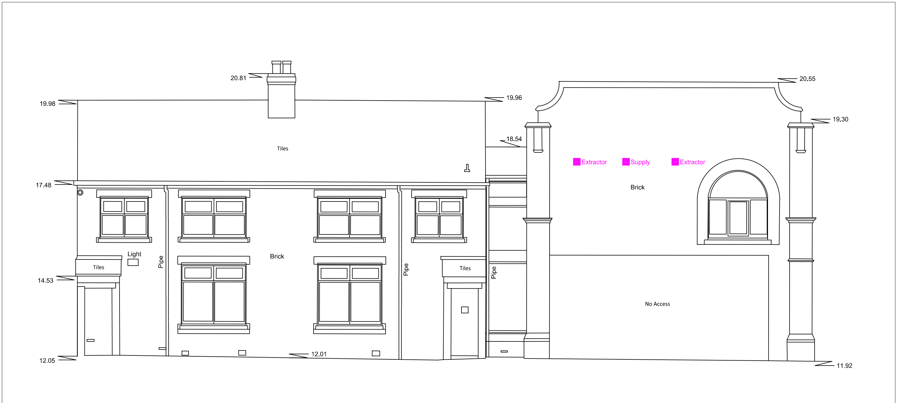
Elevation Through AA (Between Buildings)
