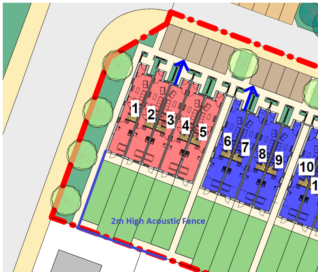
Figure 5 – Recommended location of noise barrier
