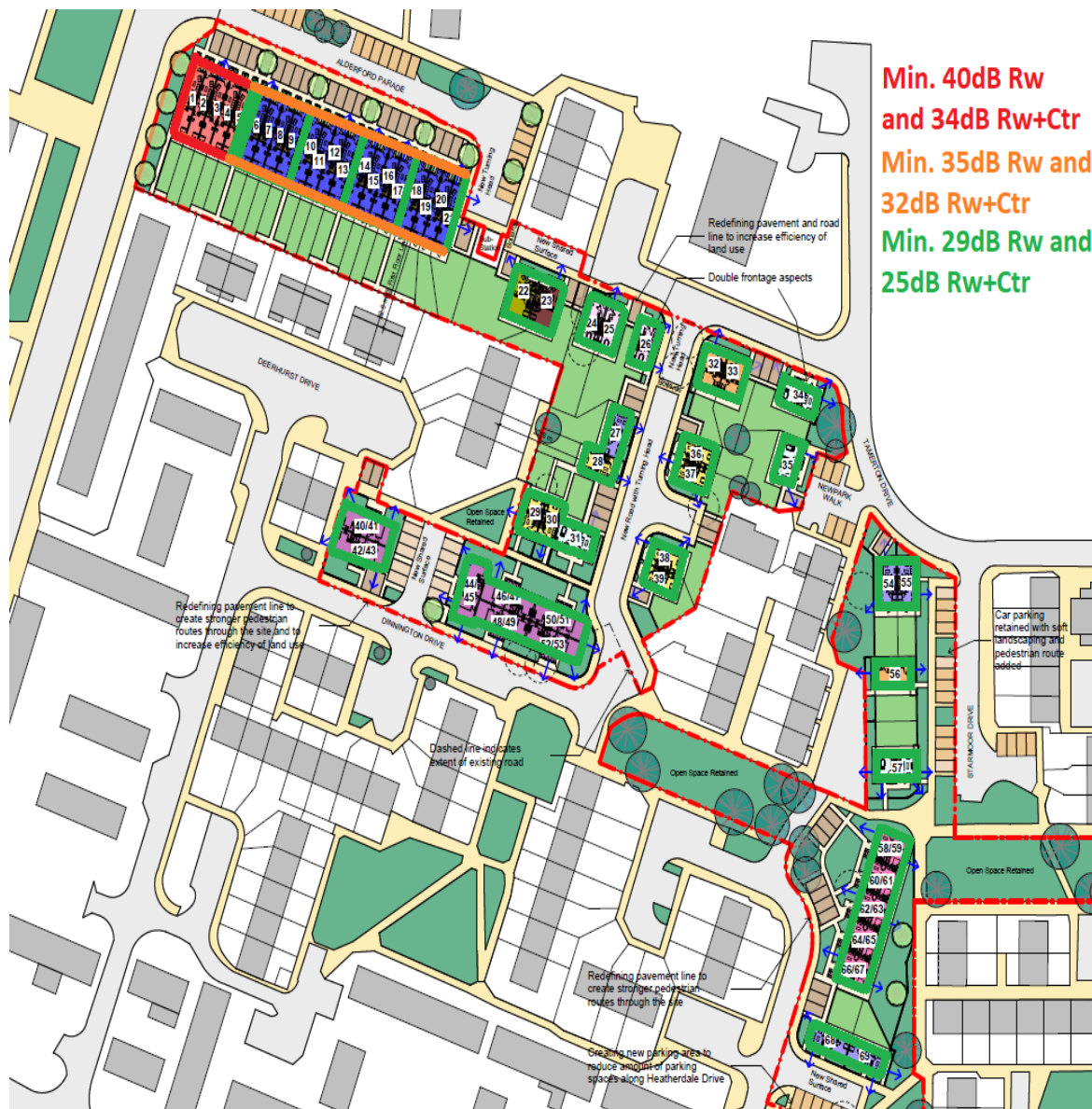
Figure 6 – Recommended glazing specification
