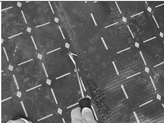
Probe testing hand welded membrane lap joints
