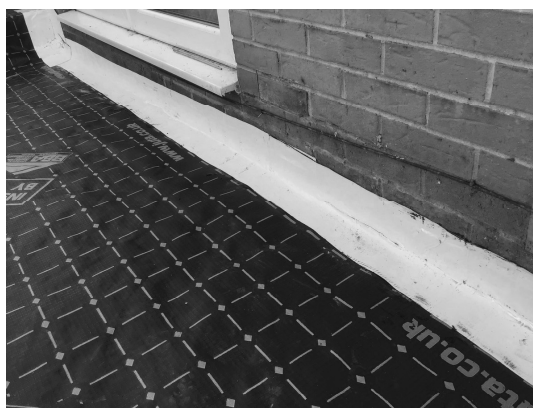
Retro fit detailing sealing the membrane onto the pre primed existing wall using Juta GP SAM
