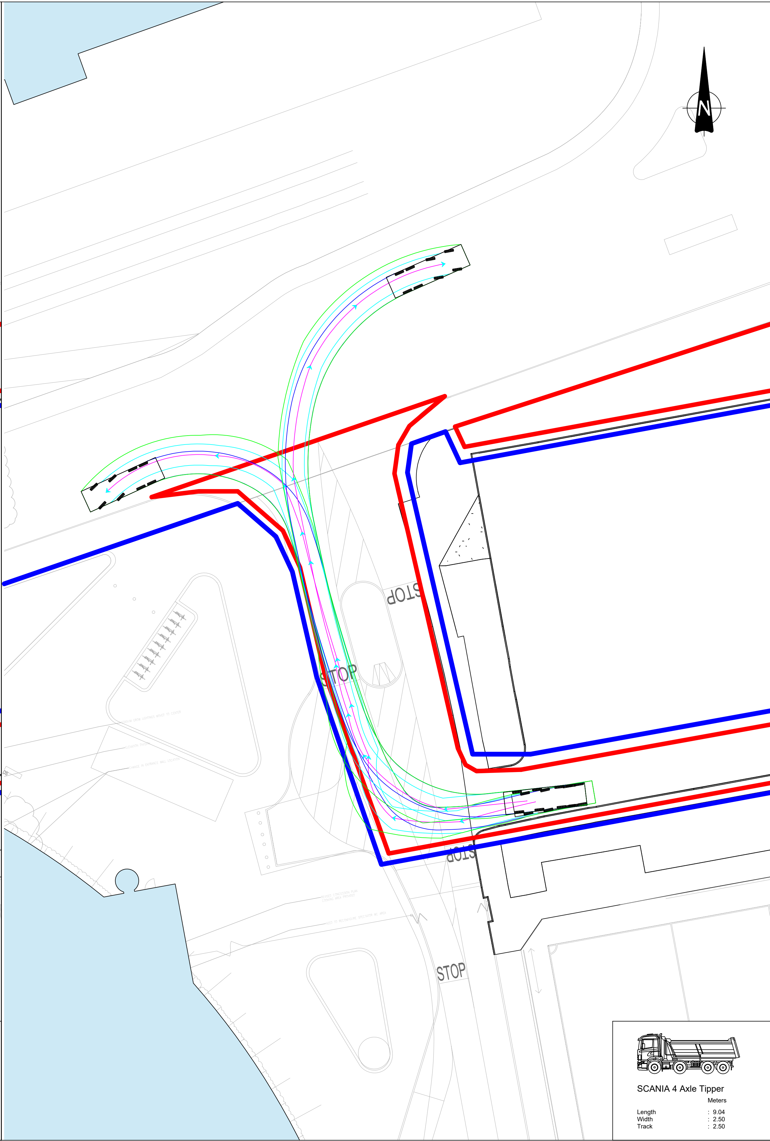
VEHICLE EGRESS 1:250 @ A1 1:500 @ A3
