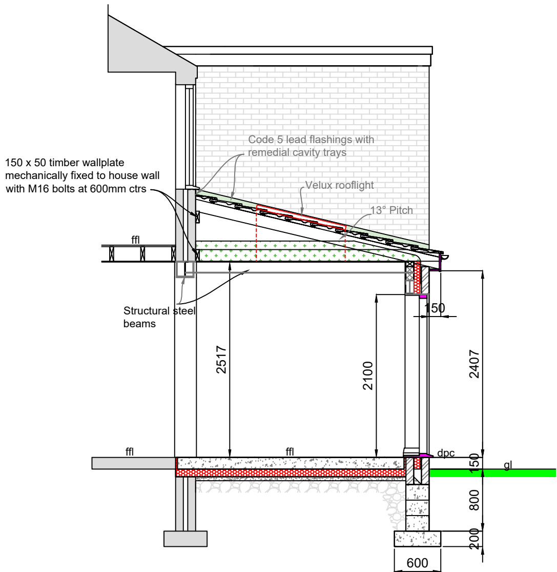
Cross Section Thro' Kitchen
