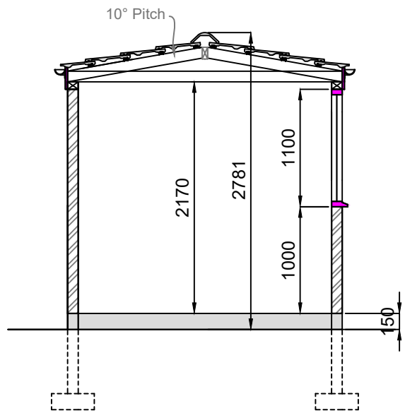
Cross Section Thro' Store Rooms
