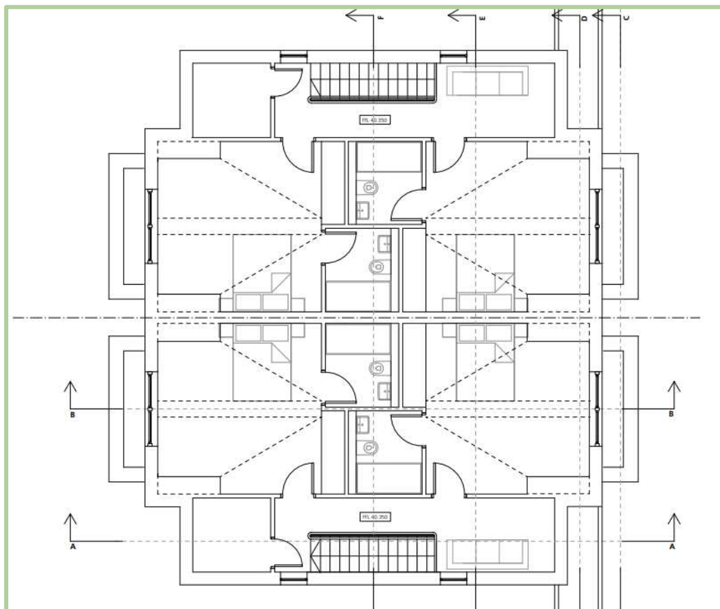
Figure 2.5 – Proposed Second Floor Plans
