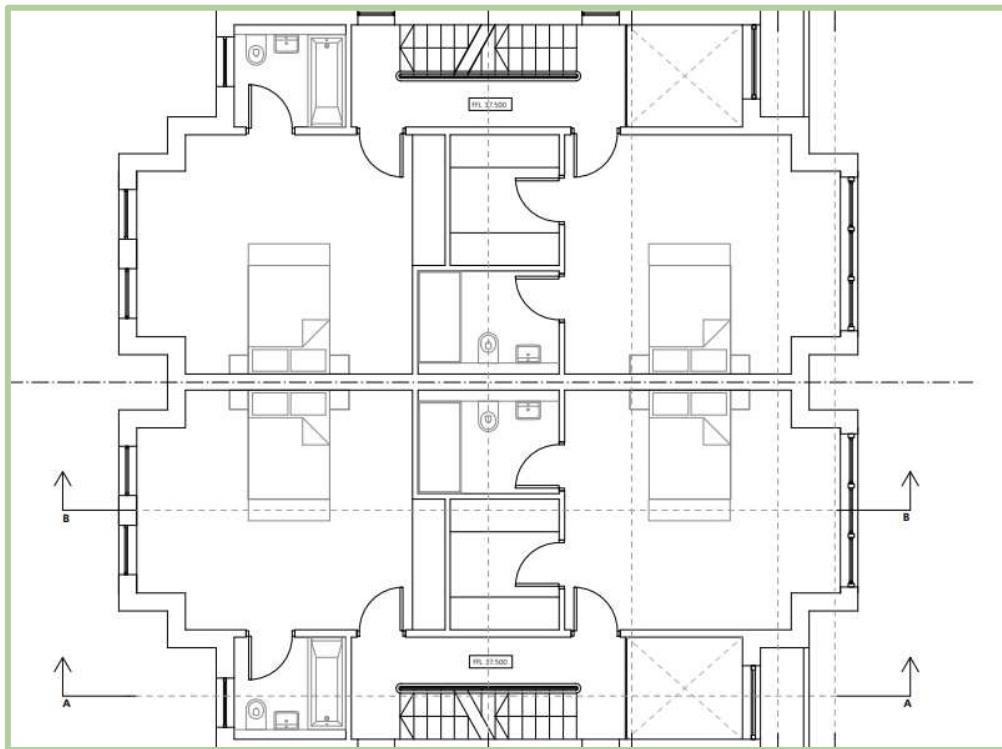
Figure 2.5 – Proposed Second Floor Plans
