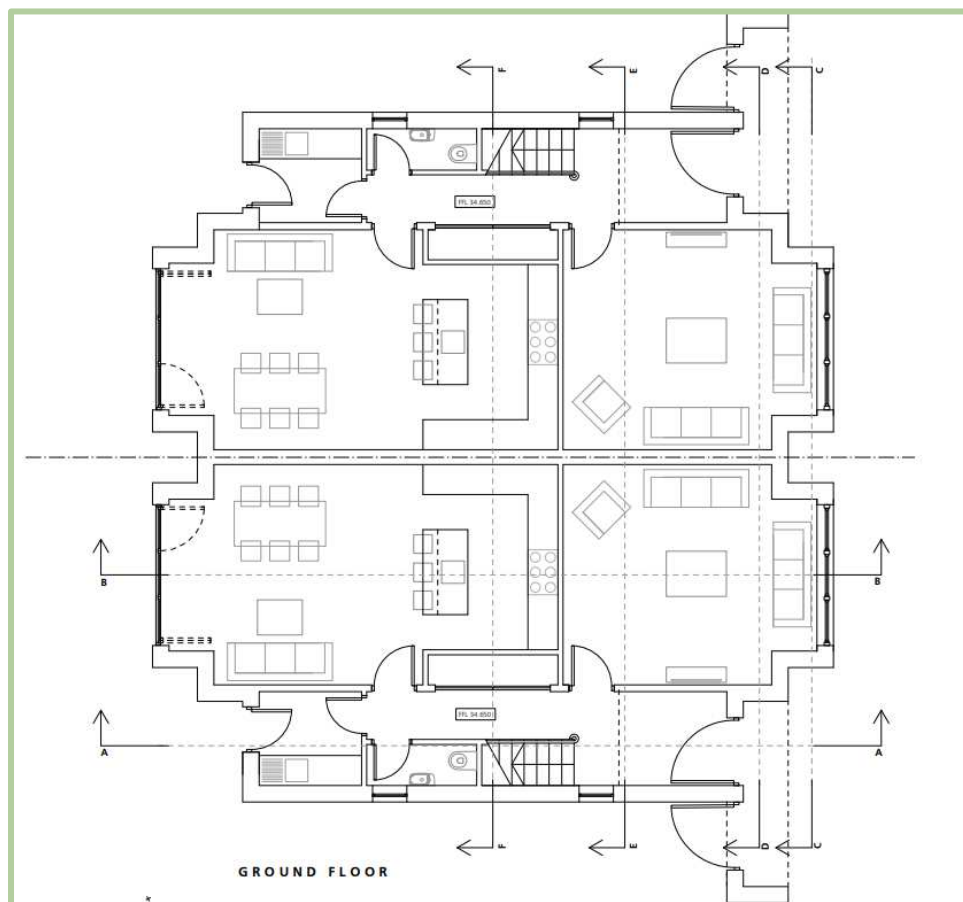
Figure 2.3 – Proposed Ground Floor Plans
