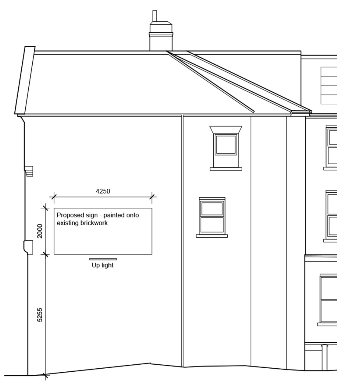
1. Sign elevation 1:100
