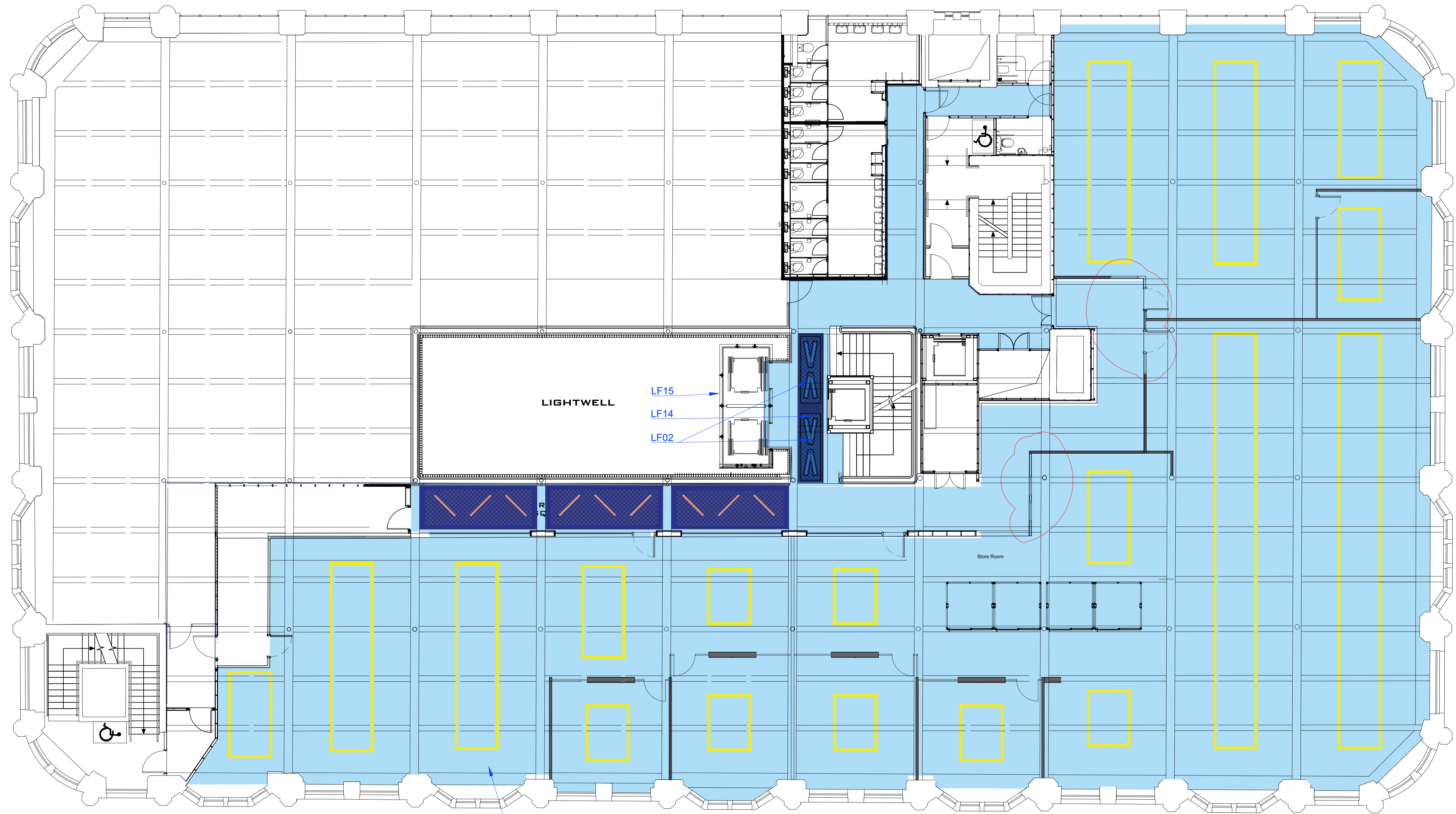
First Floor - Reflective Ceiling Plan Scale 1:100
