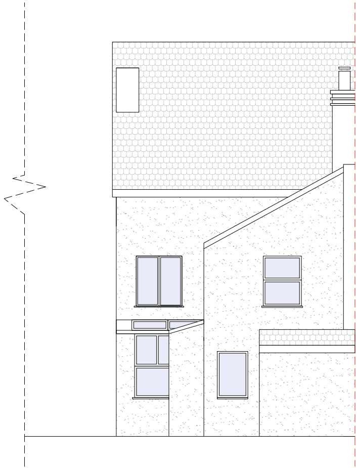
Proposed East Elevation (no proposed change)
