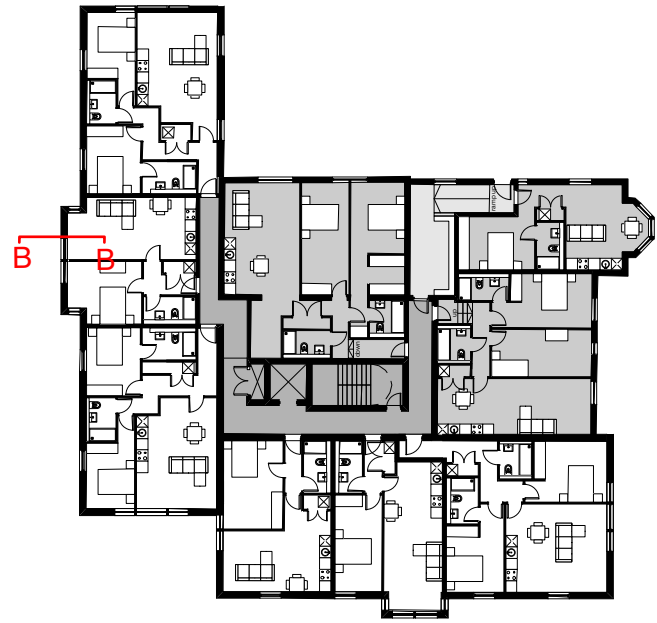
KEY PLAN - UPPER GROUND FLOOR 1:400@A1
