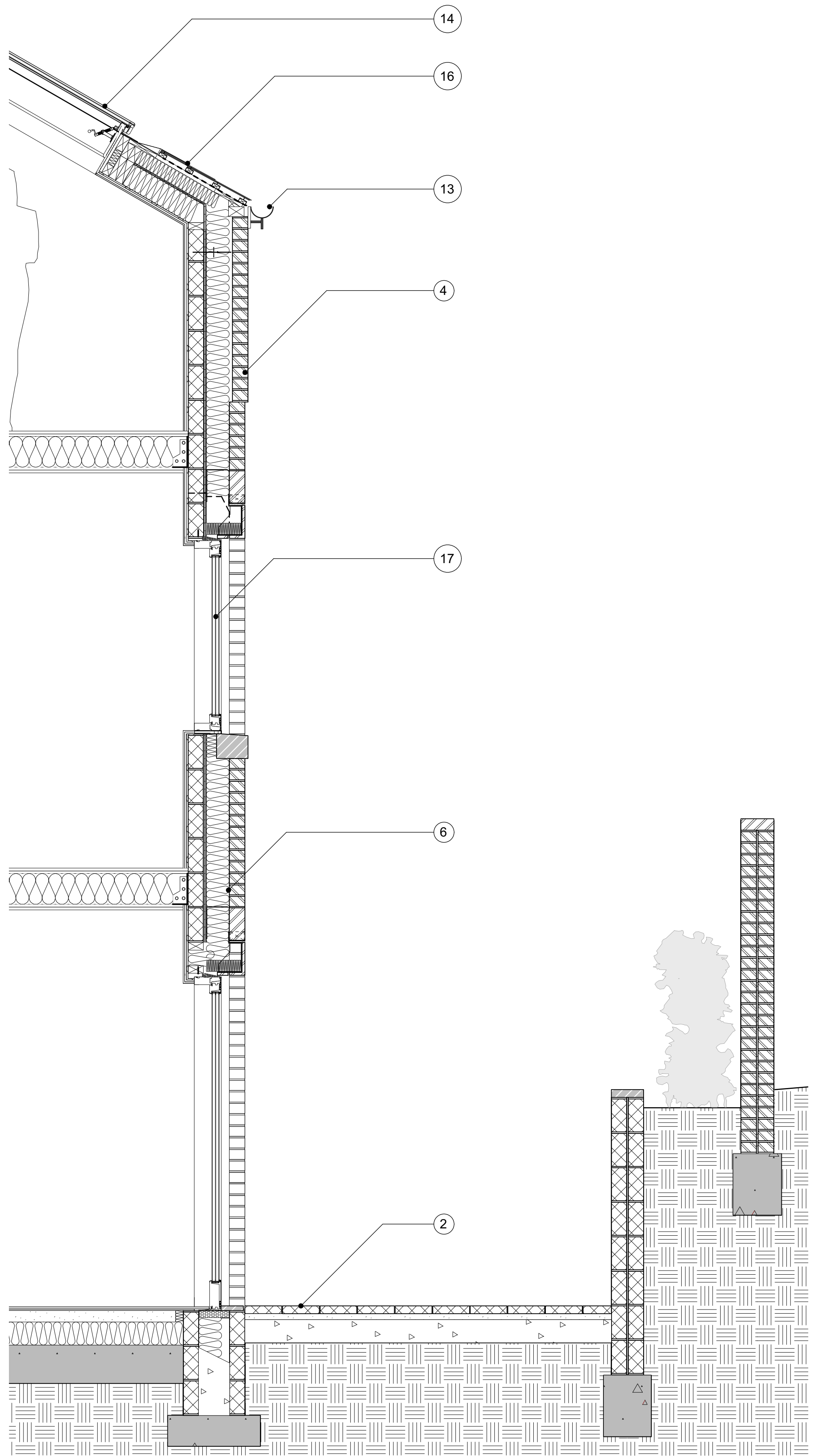
DETAIL SECTION BB 1:20@A1
