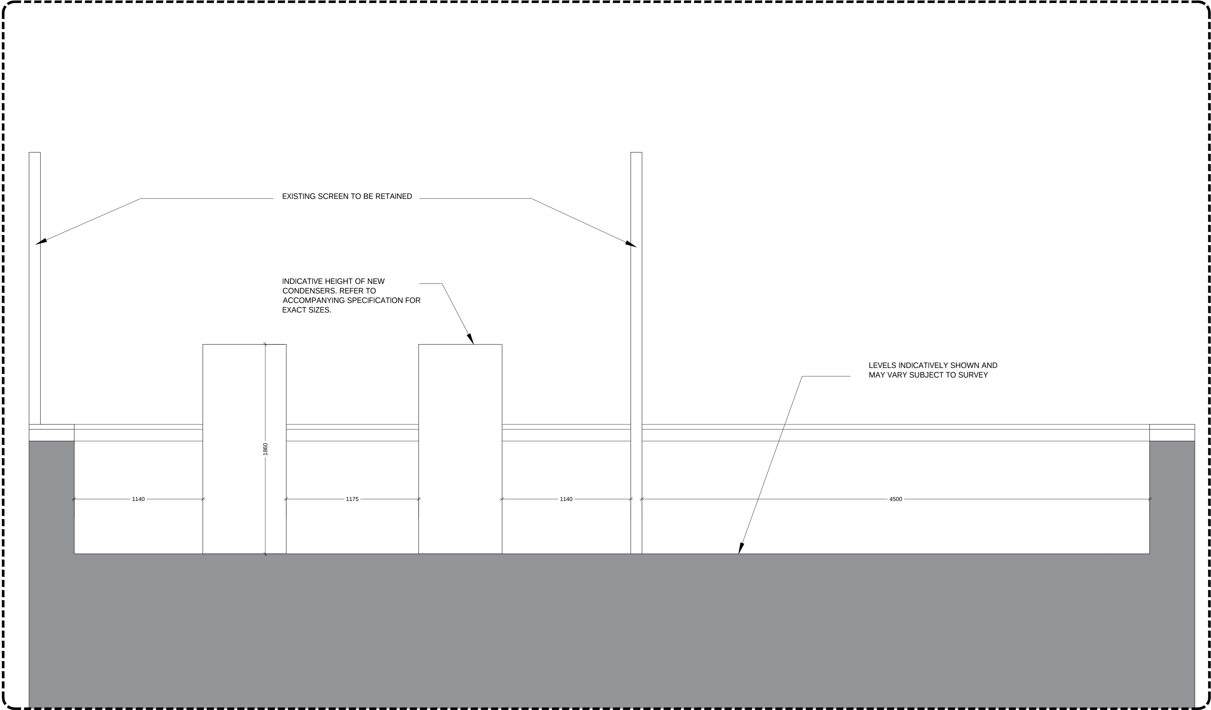
02 EXISTING / PROPOSED SECTION - PLANT DECK TO REMAIN AS EXISTING WITH SOME CONDENSERS BEING REPLACED 10002 SCALE: 1:20 @ A1
