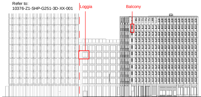
Key Elevation - South
