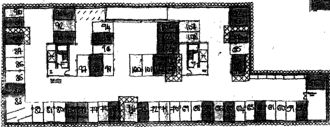
1 Lower Basement Floor Scale Drawing based on 1970 floor plans
