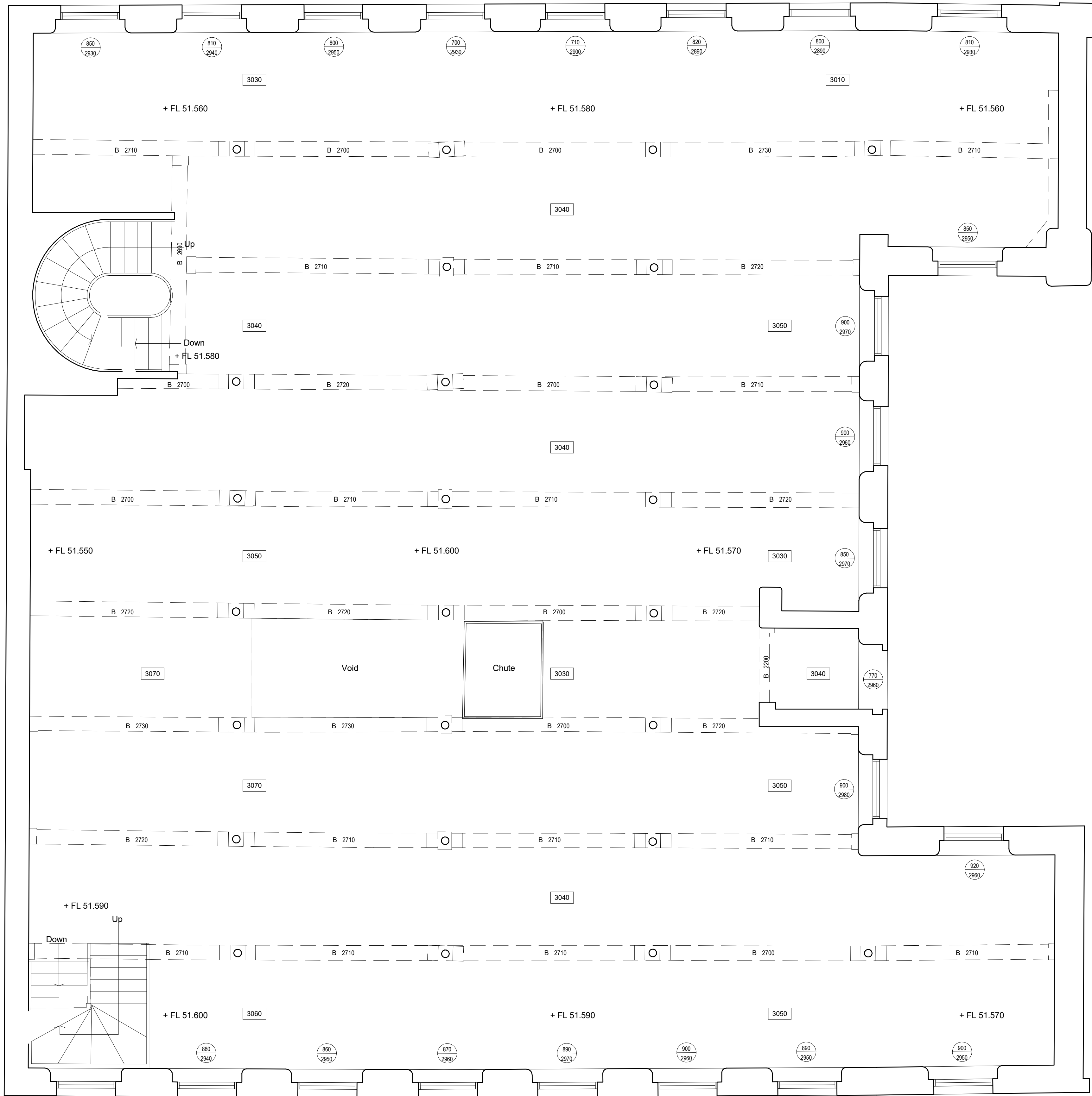
1 | Second floor - existing.
