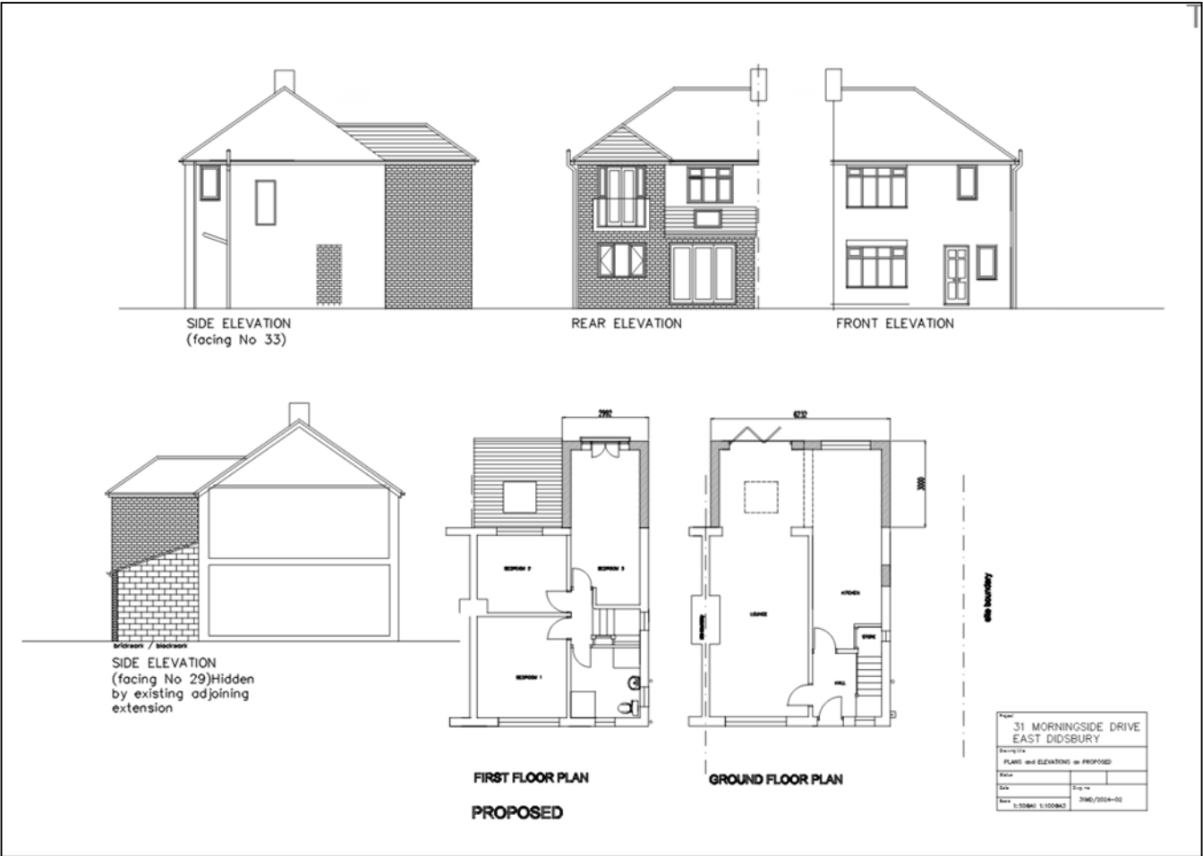
Figure 2. Proposed plan and elevation
