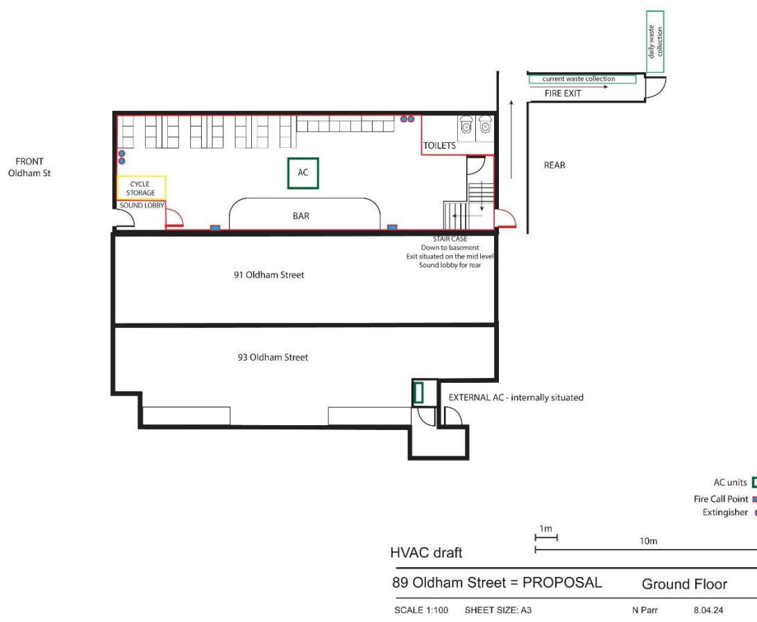
Figure 3: Location of air conditioning plant
