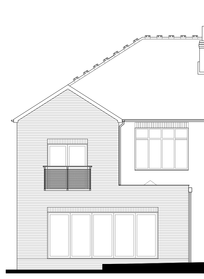
REAR ELEVATION
