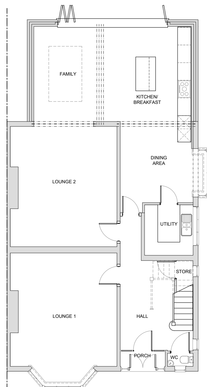
GROUND FLOOR
