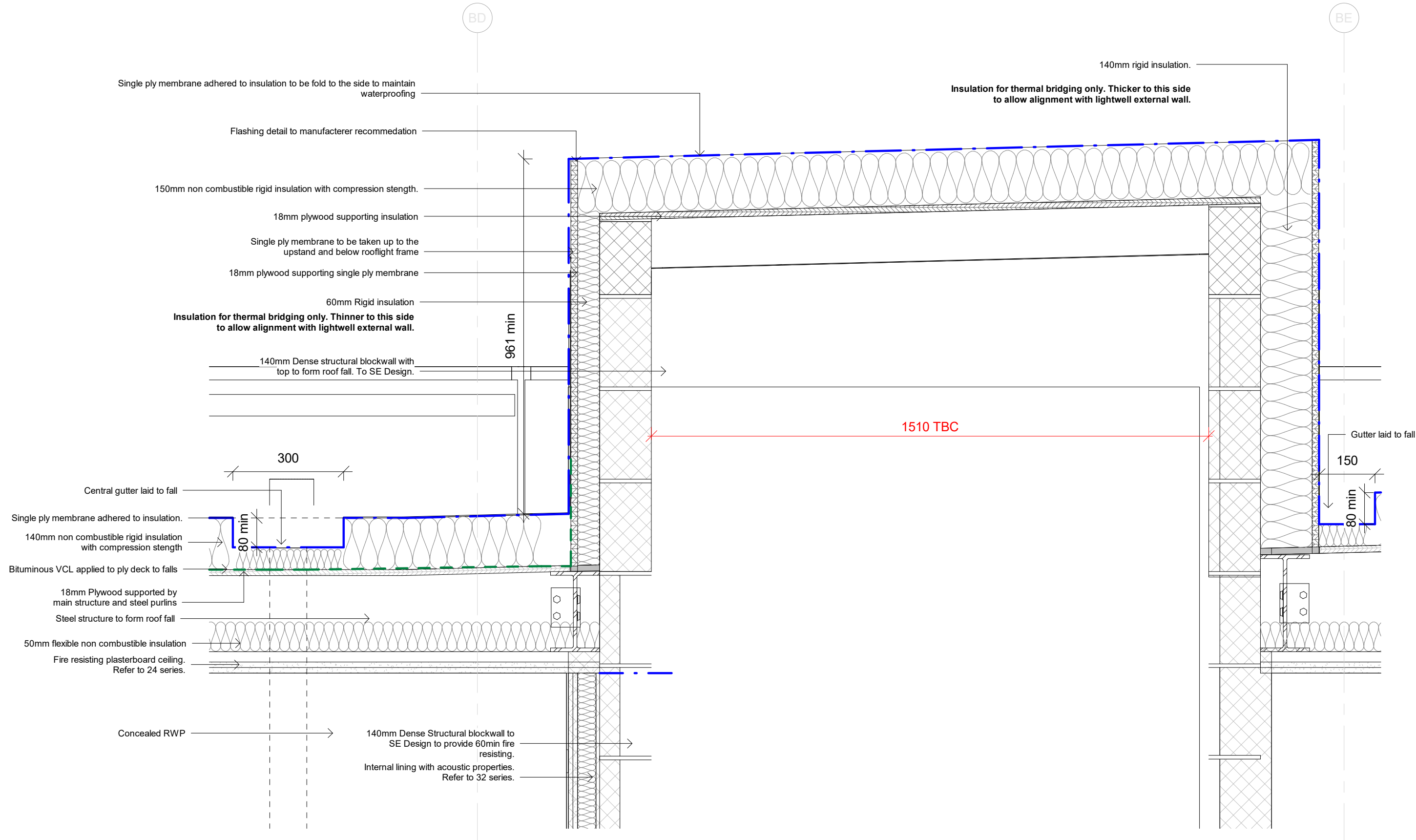
2 | Roof Details - Lift overrun_Cross section.
