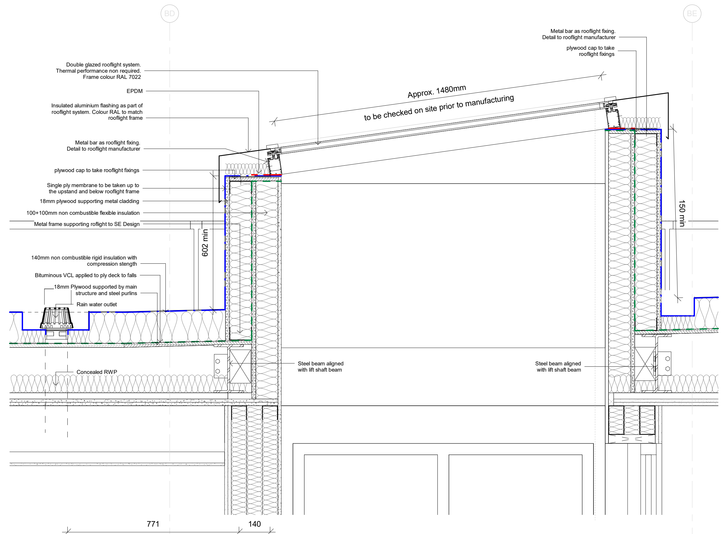
3 | Roof details - Rooflight cross section.
