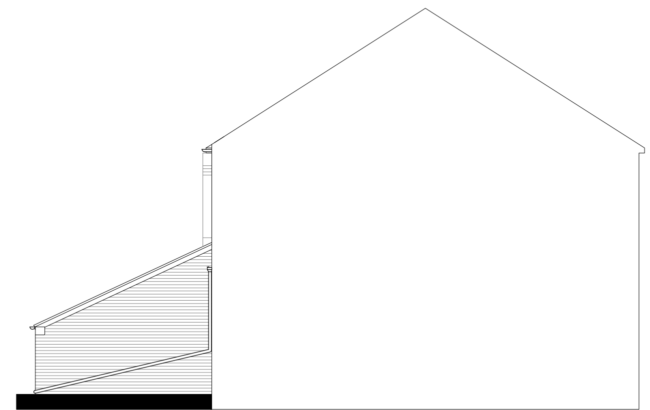
SIDE ELEVATION
