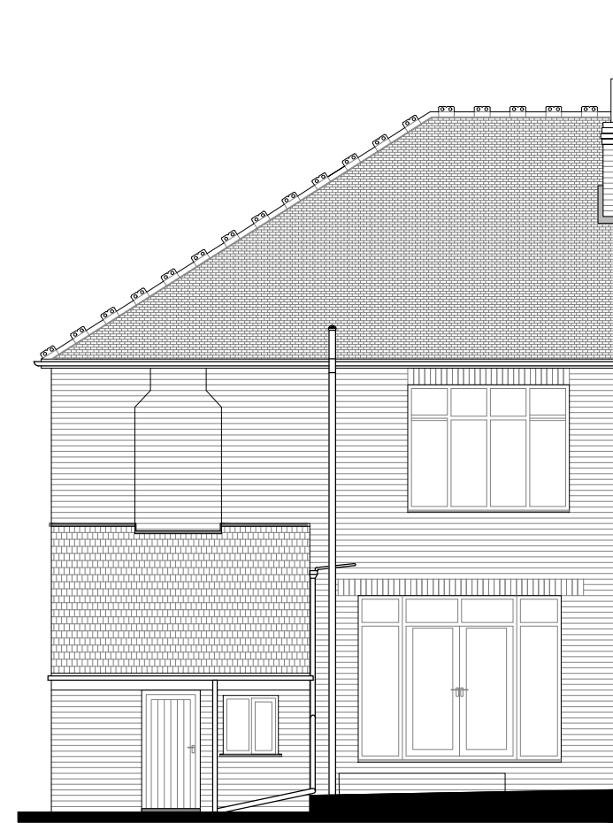
REAR ELEVATION
