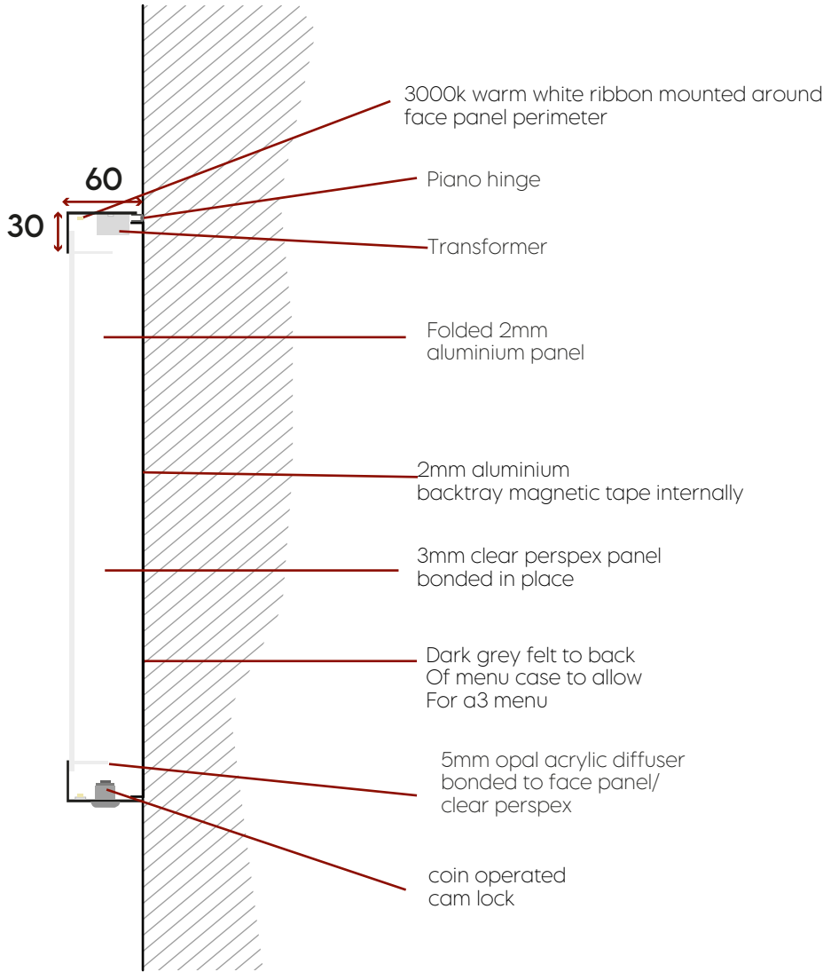
Side section 1:5 scale
