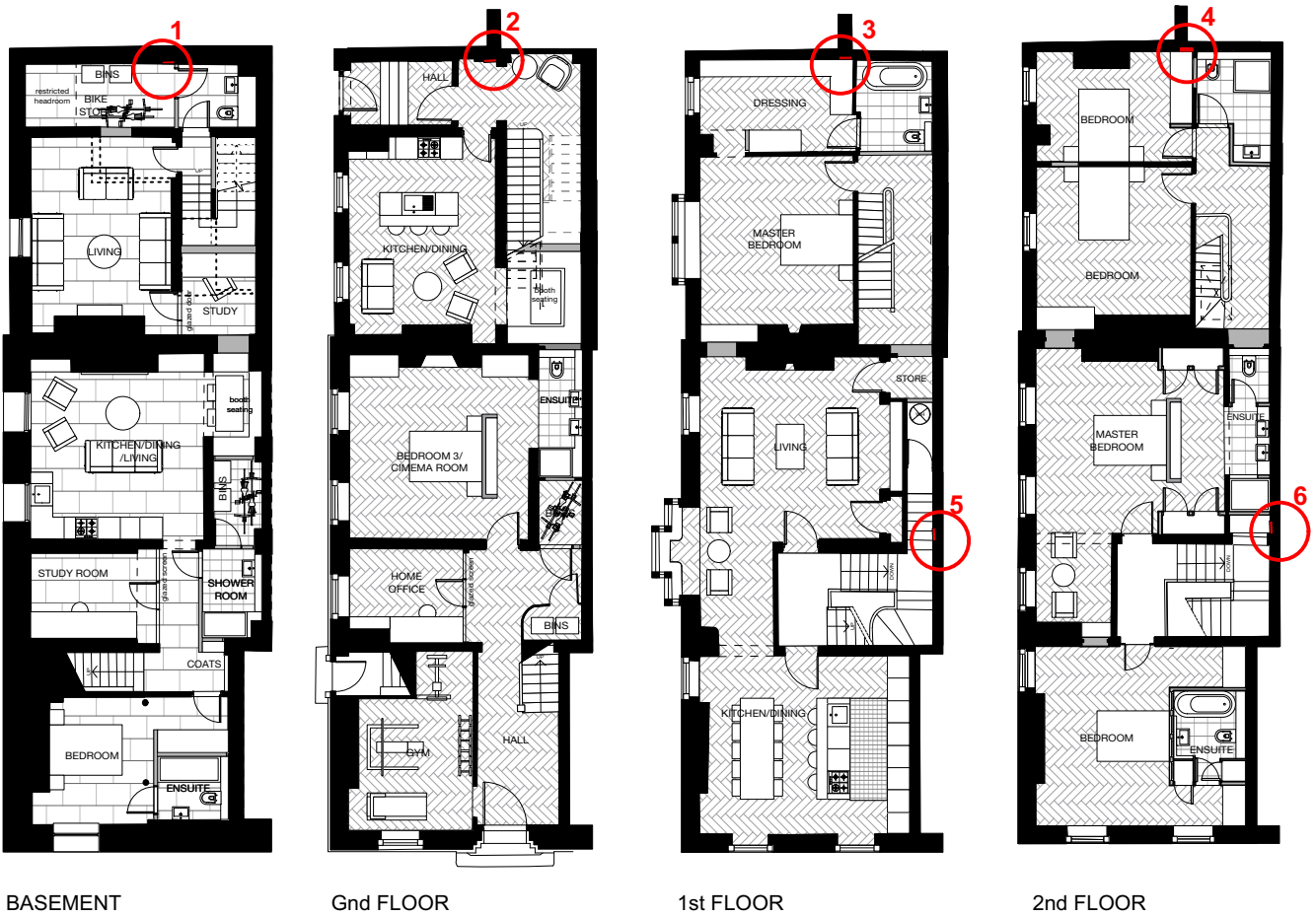
KEY PLAN TO SOIL PIPE LOCATIONS:
