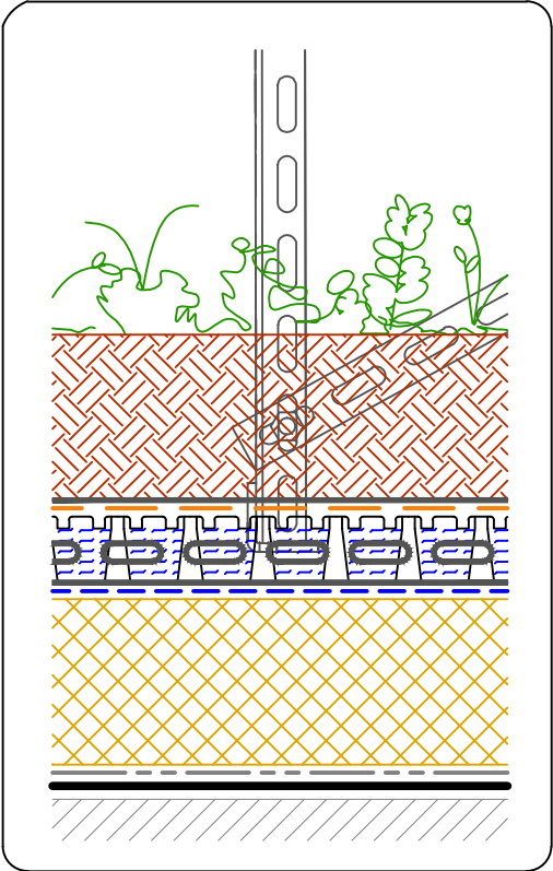
Layer Build-up - Scale 1:5
