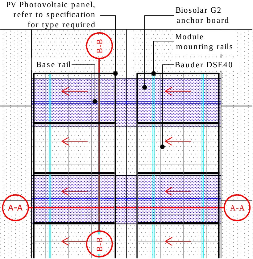
Bauder Biosolar Module Section - Top Elevation - Scale 1:50
