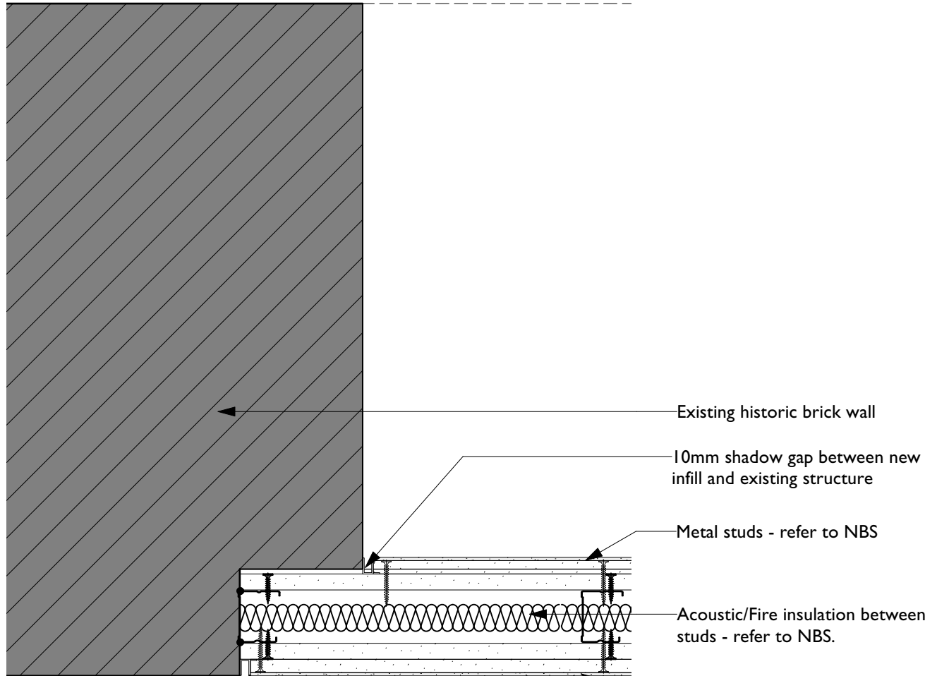
2 Partition Type A - Detail - see drawings I22 and I23 Scale: 1:5
