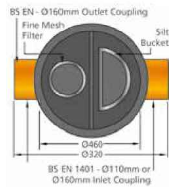
SILT TRAP DETAIL
