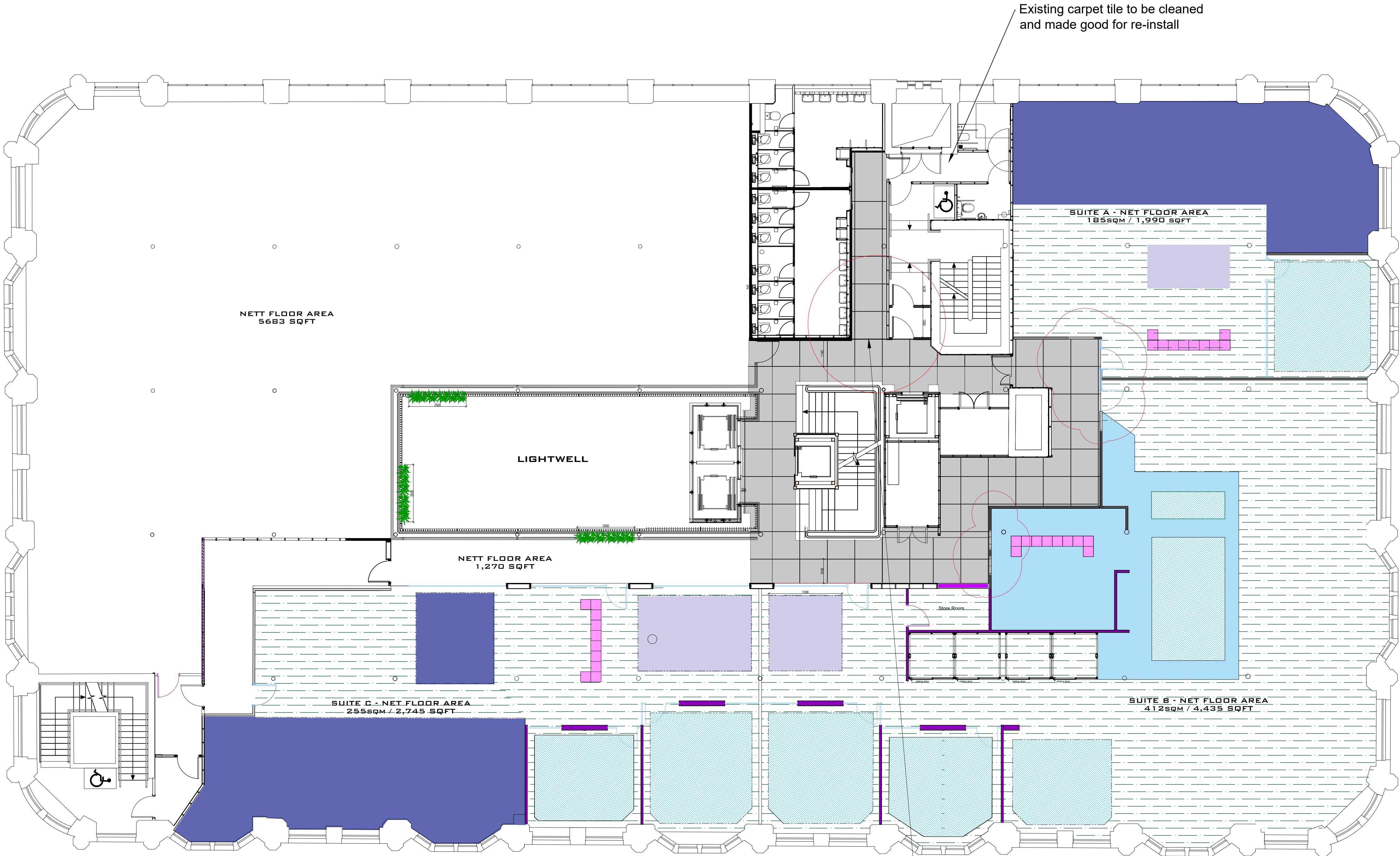
First Floor - Floor Finishes Scale 1:100
