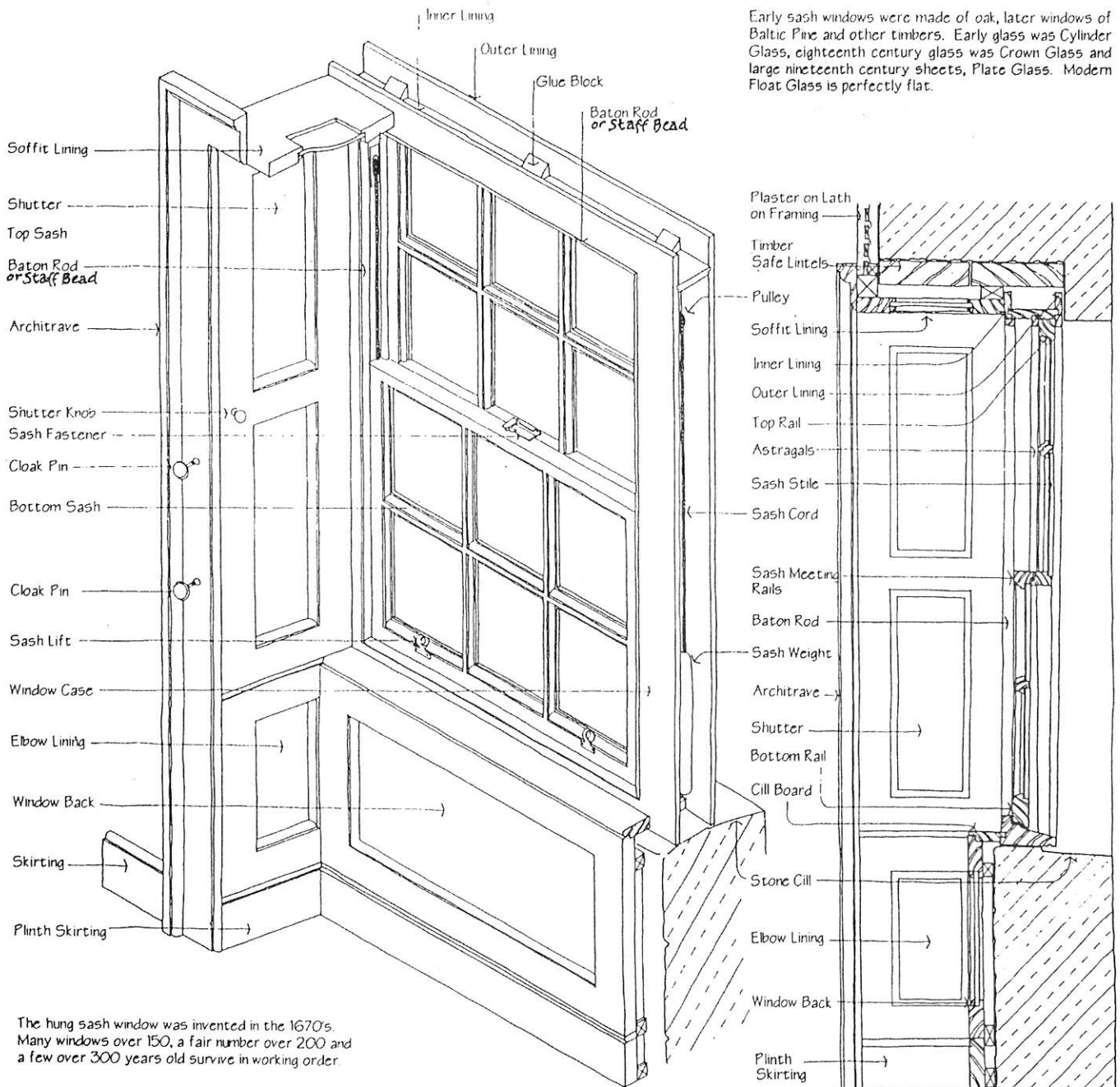
Section Through Window
