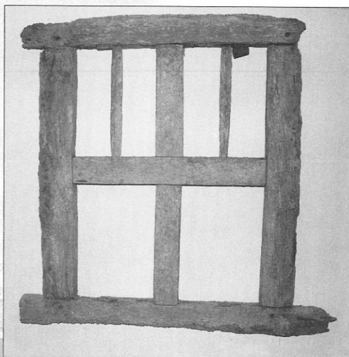
17 th century oak window frame from Ville a L'Eveque, Trinity, now held in the Jersey Museum
