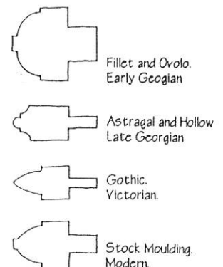
Glazing Bars or Astragals
