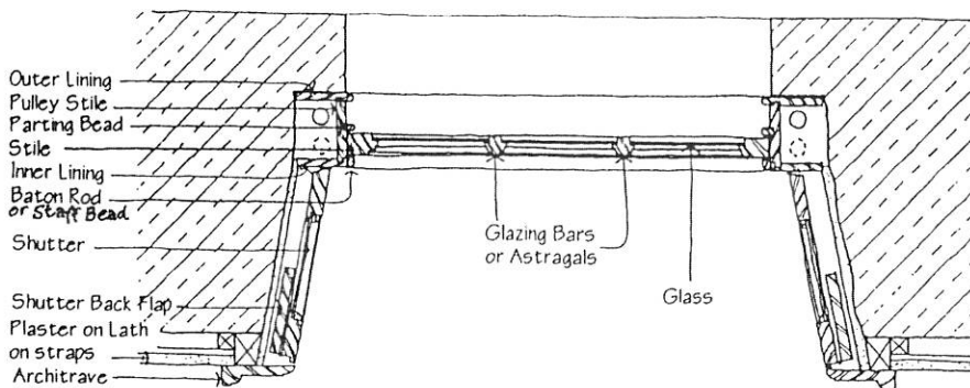
Plan Section Through Window
