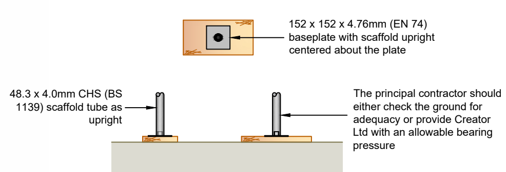
FOUNDATION DETAIL 225 x 38 x 450mm (BS EN 2482) Scaffold Board Solepad Scale - 1:25
