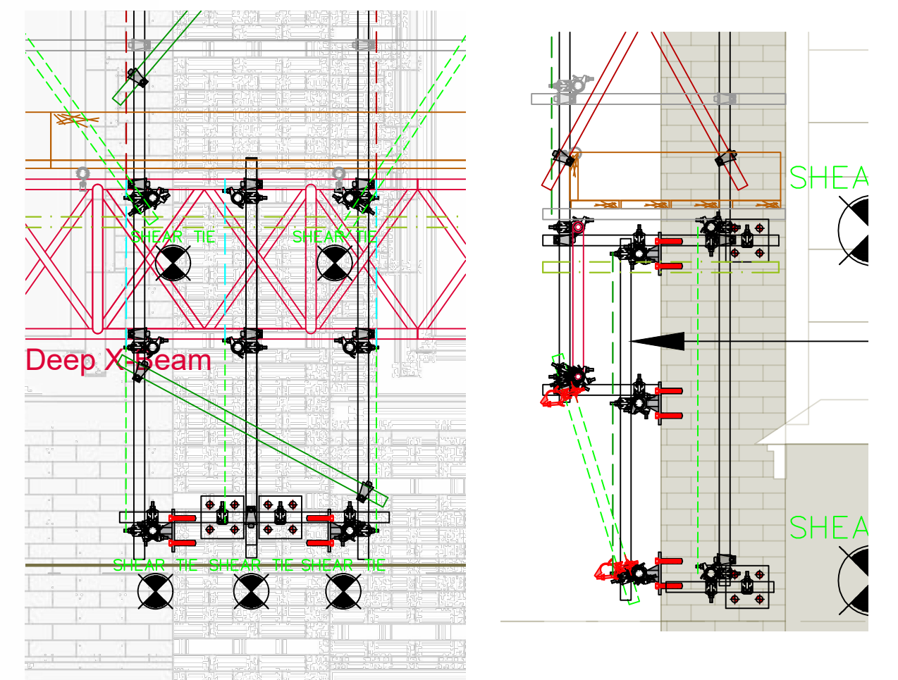
GALLOWS BRACKET DETAIL scale 1:25
