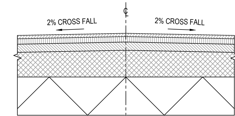
TYPICAL SECTION THROUGH ACCESS ROAD [SCALE: 1:20]
