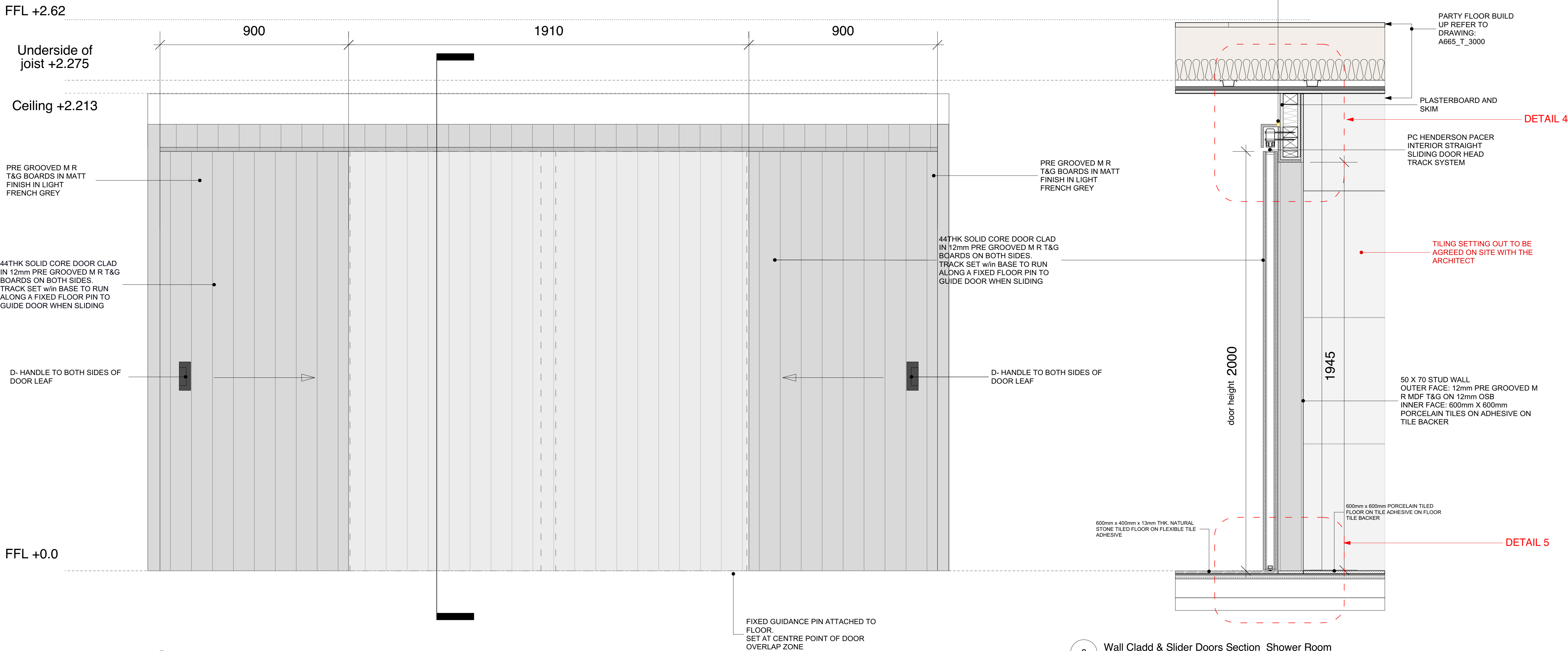
2 Wall Cladd & Slider Doors Elevation_Shower Room Scale: 1:10
