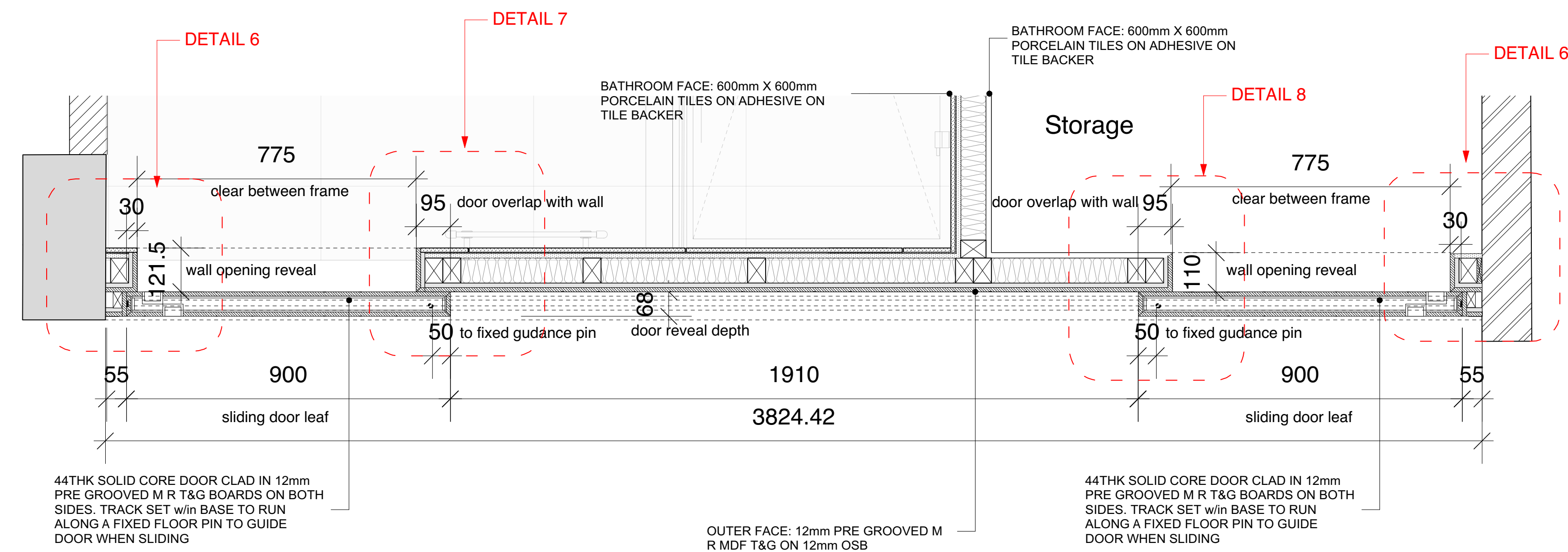
1 Basement Shower Room Detail Plan Scale: 1:10
