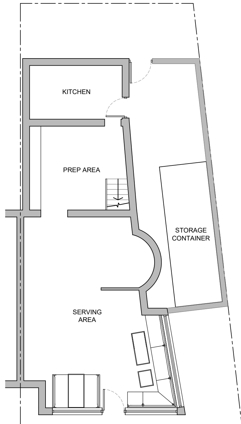
GROUND FLOOR
