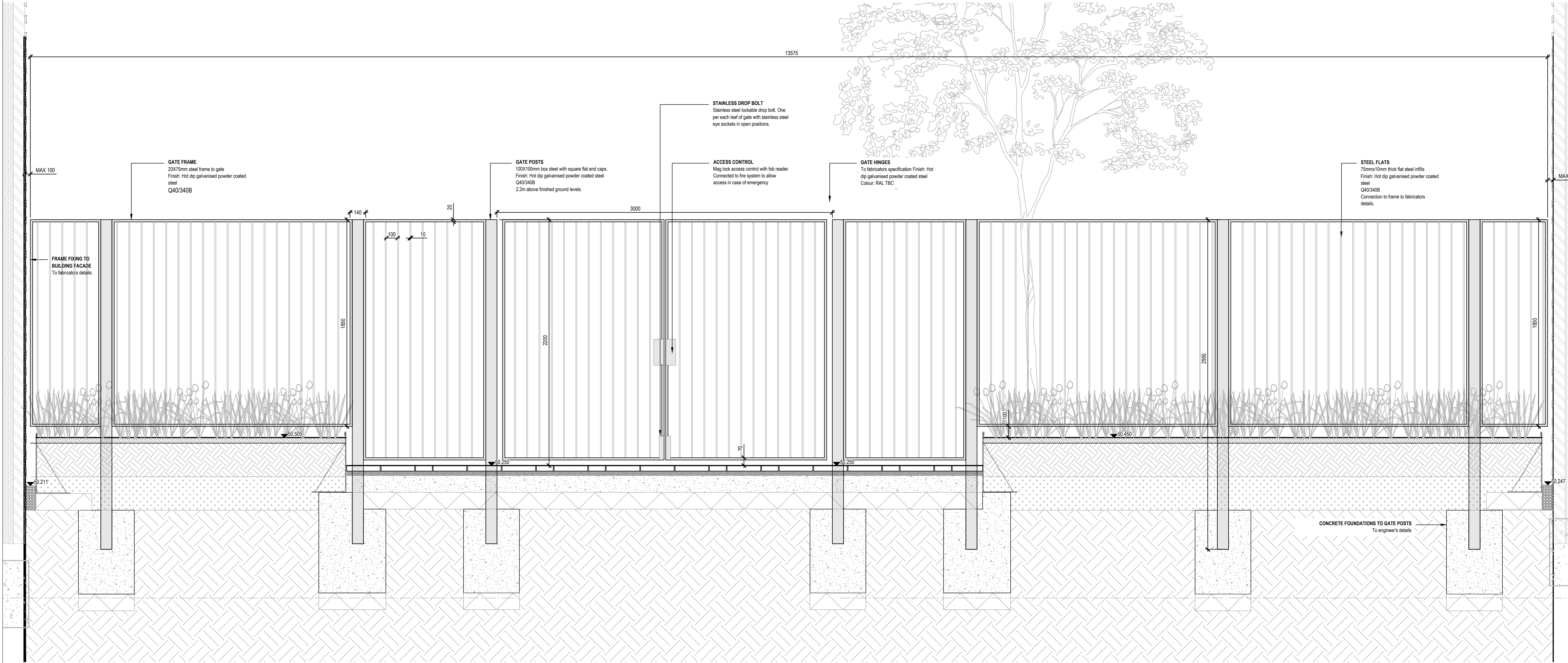
01 900331 B3 - Steel Fenceline and Pedestrian Entrance Access Scale 1: 20 @A1
